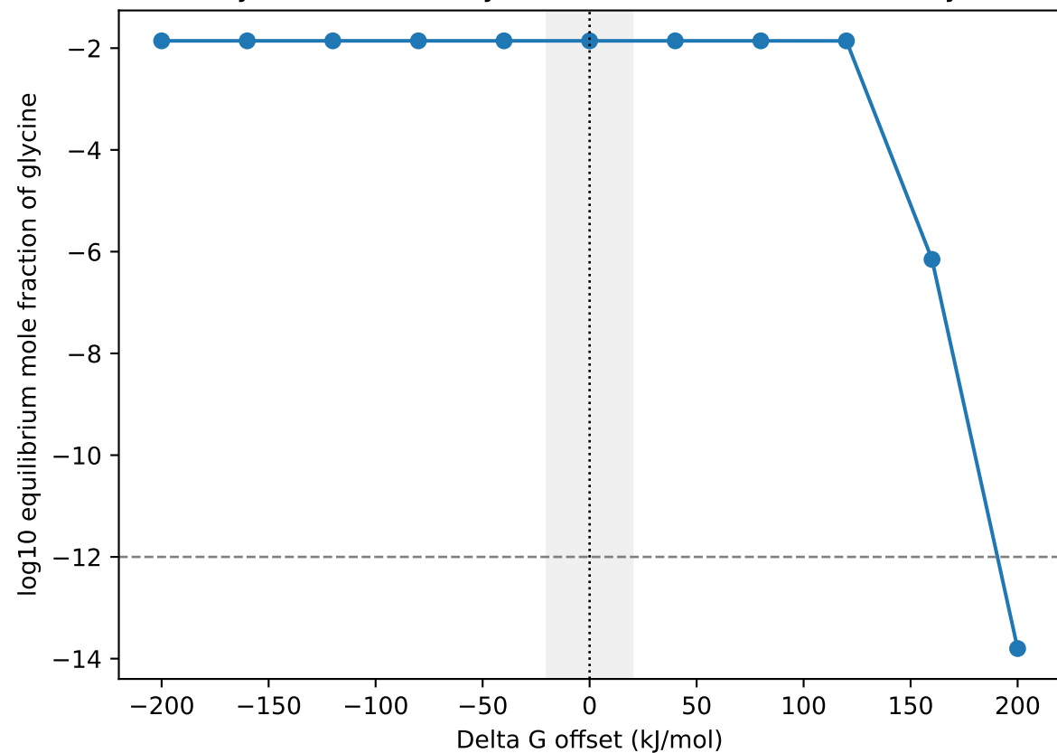
Glycine accessibility vs Gibbs offset (fixed inventory)
