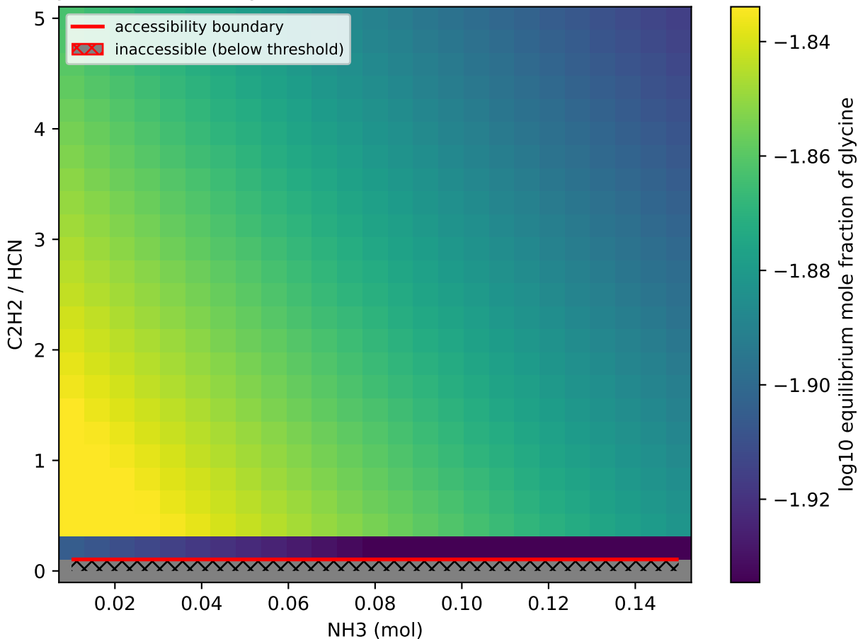
Glycine accessibility — NH 3 vs C 2 H 2 /HCN (0 C) (autoscaled)
