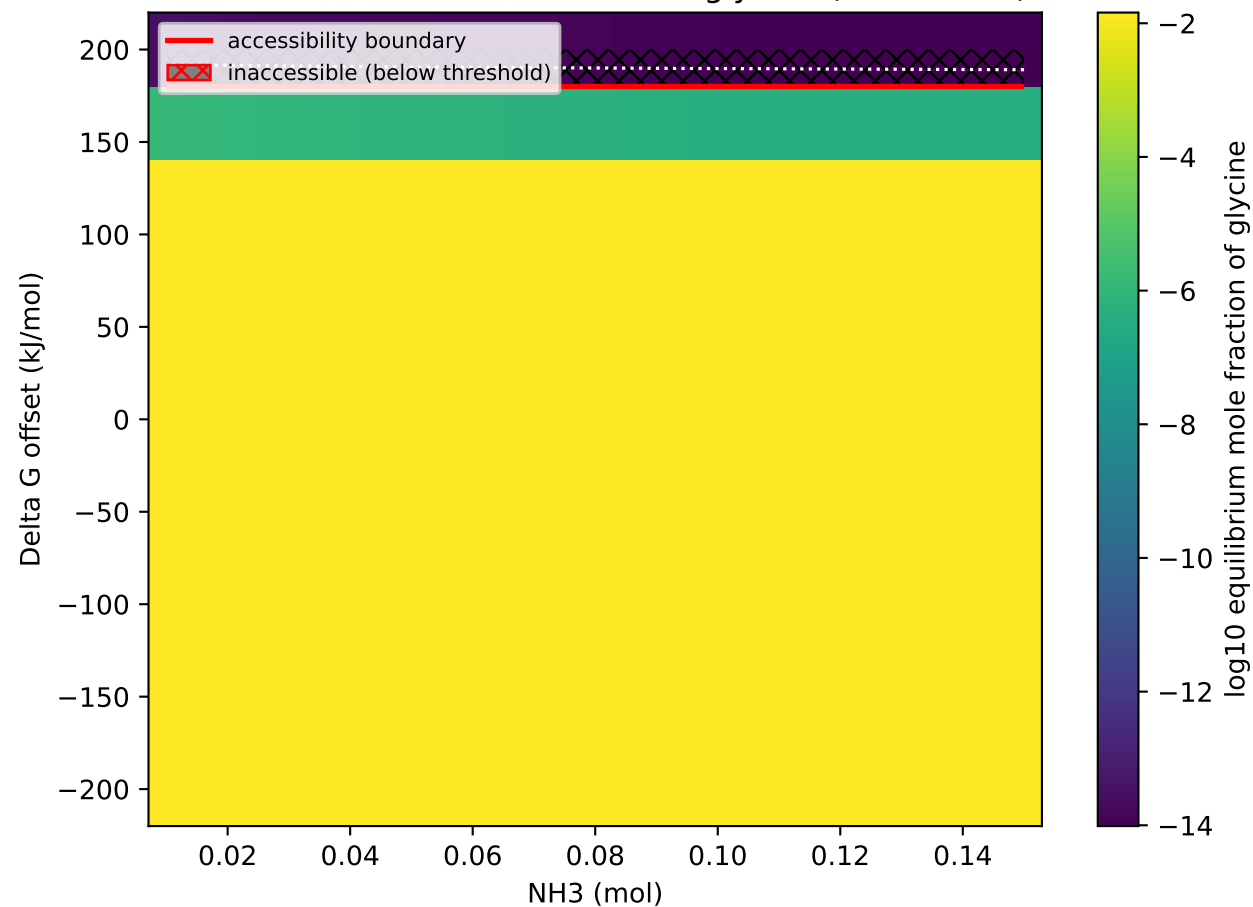
NH3 threshold vs Gibbs offset for glycine (autoscaled)
