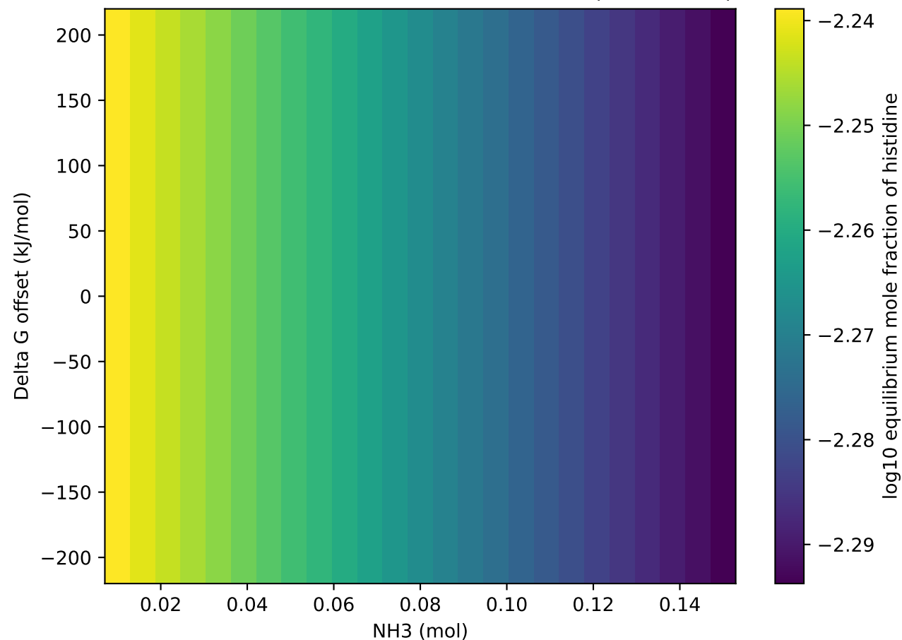
NH3 threshold vs Gibbs offset for histidine (autoscaled)
