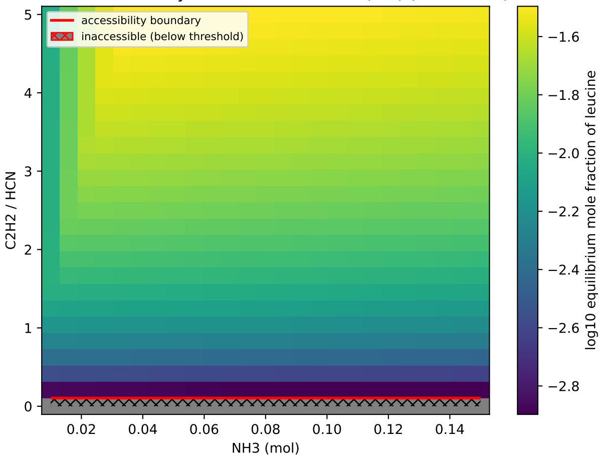
Leucine accessibility — \text{NH}_3 vs \text{C}_2\text{H}_2/\text{HCN} (0 C) (autoscaled)
