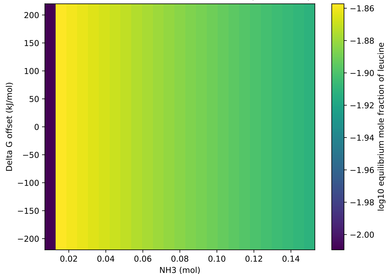
NH 3 threshold vs Gibbs offset for leucine (autoscaled)
