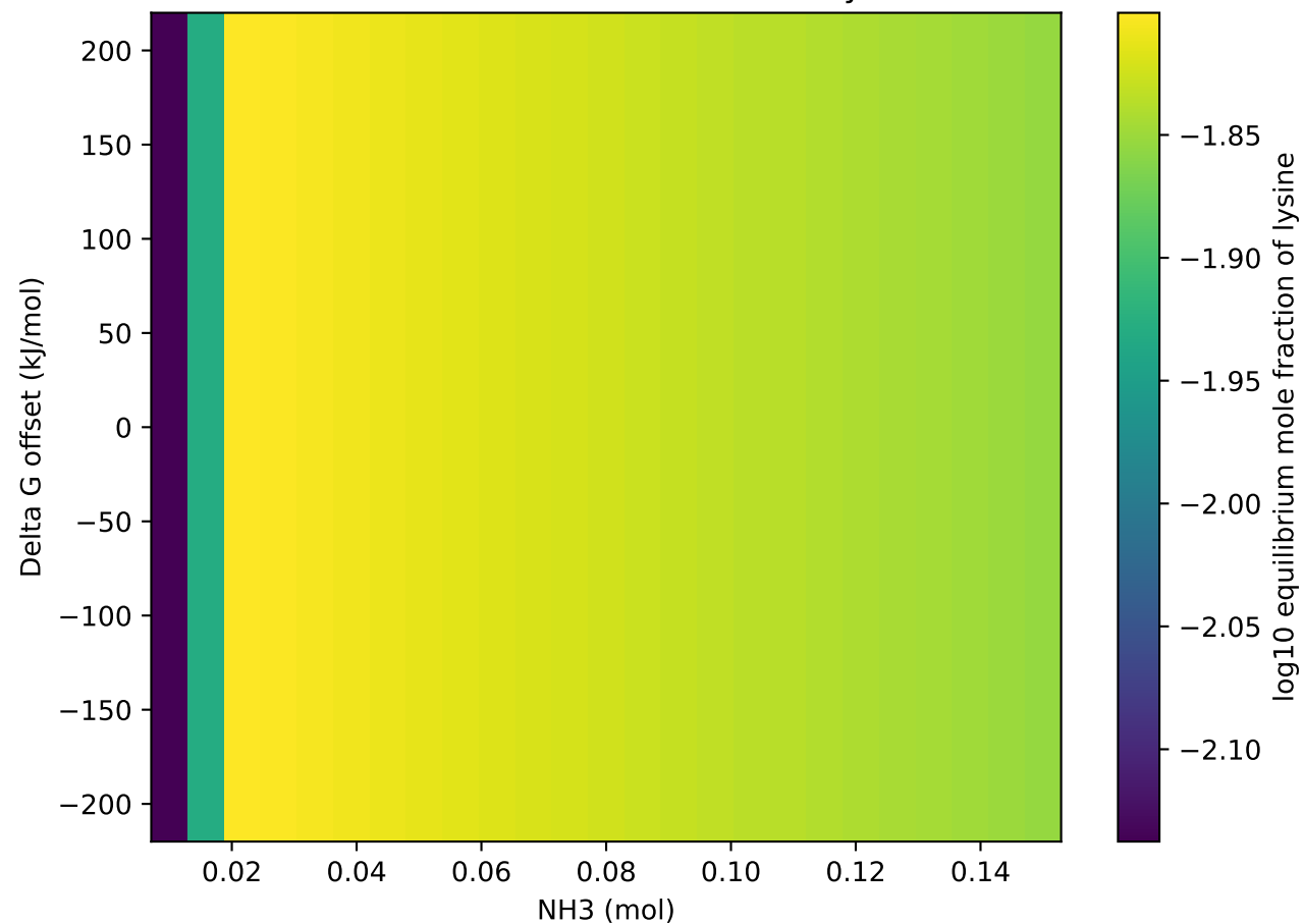
NH 3 threshold vs Gibbs offset for lysine
