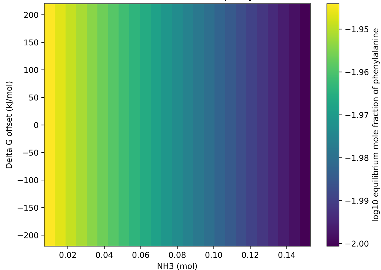
NH 3 threshold vs Gibbs offset for phenylalanine
