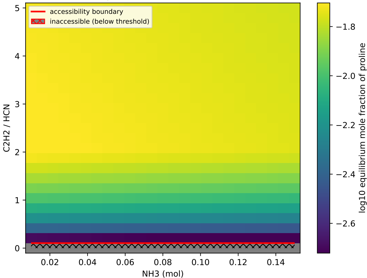
Proline accessibility — NH 3 vs C 2 H 2 /HCN (0 C) (autoscaled)
