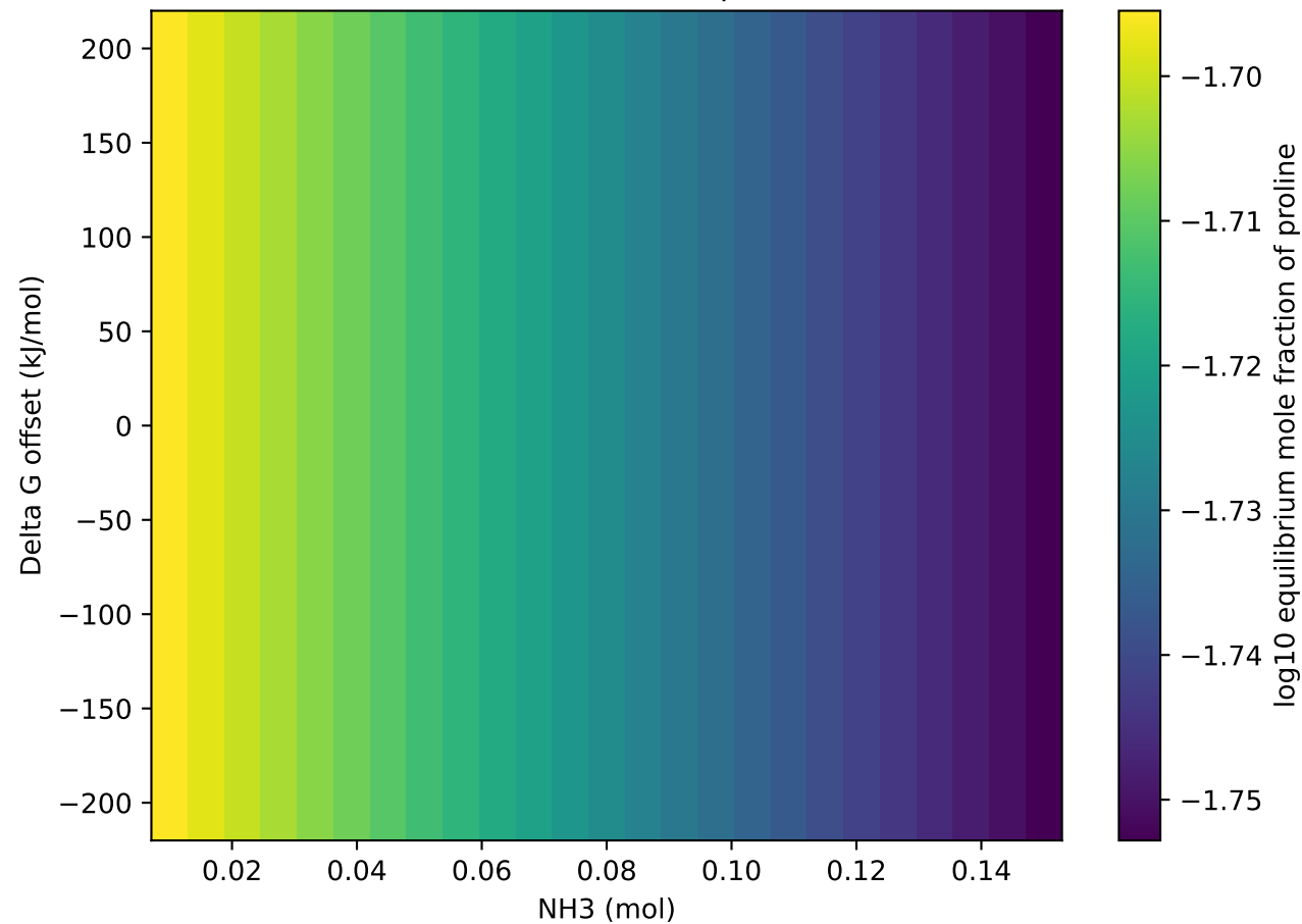
NH 3 threshold vs Gibbs offset for proline (autoscaled)
