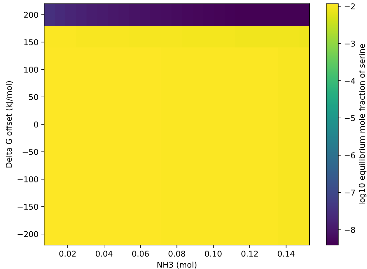
NH3 threshold vs Gibbs offset for serine (autoscaled)
