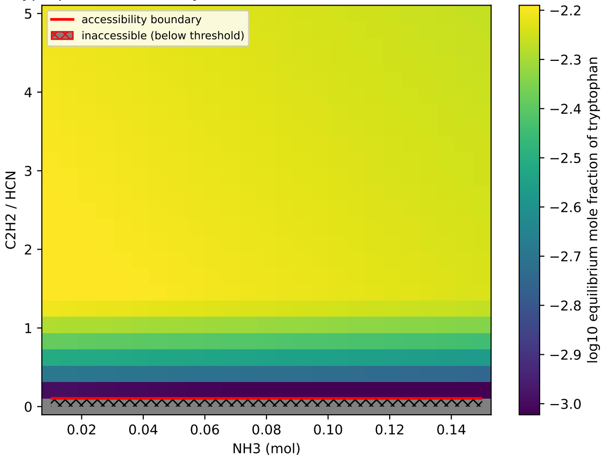
Tryptophan accessibility — \text{NH}_3 vs \text{C}_2\text{H}_2/\text{HCN} (0 C) (autoscaled)
