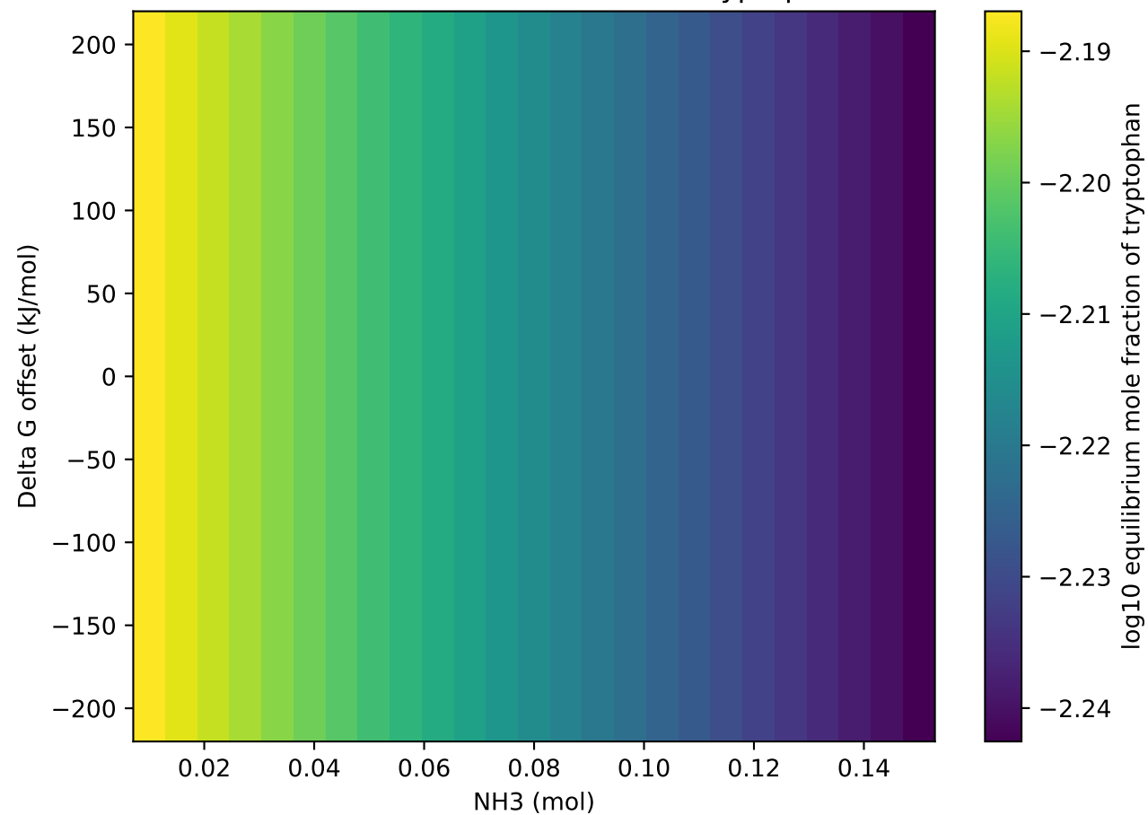
NH 3 threshold vs Gibbs offset for tryptophan
