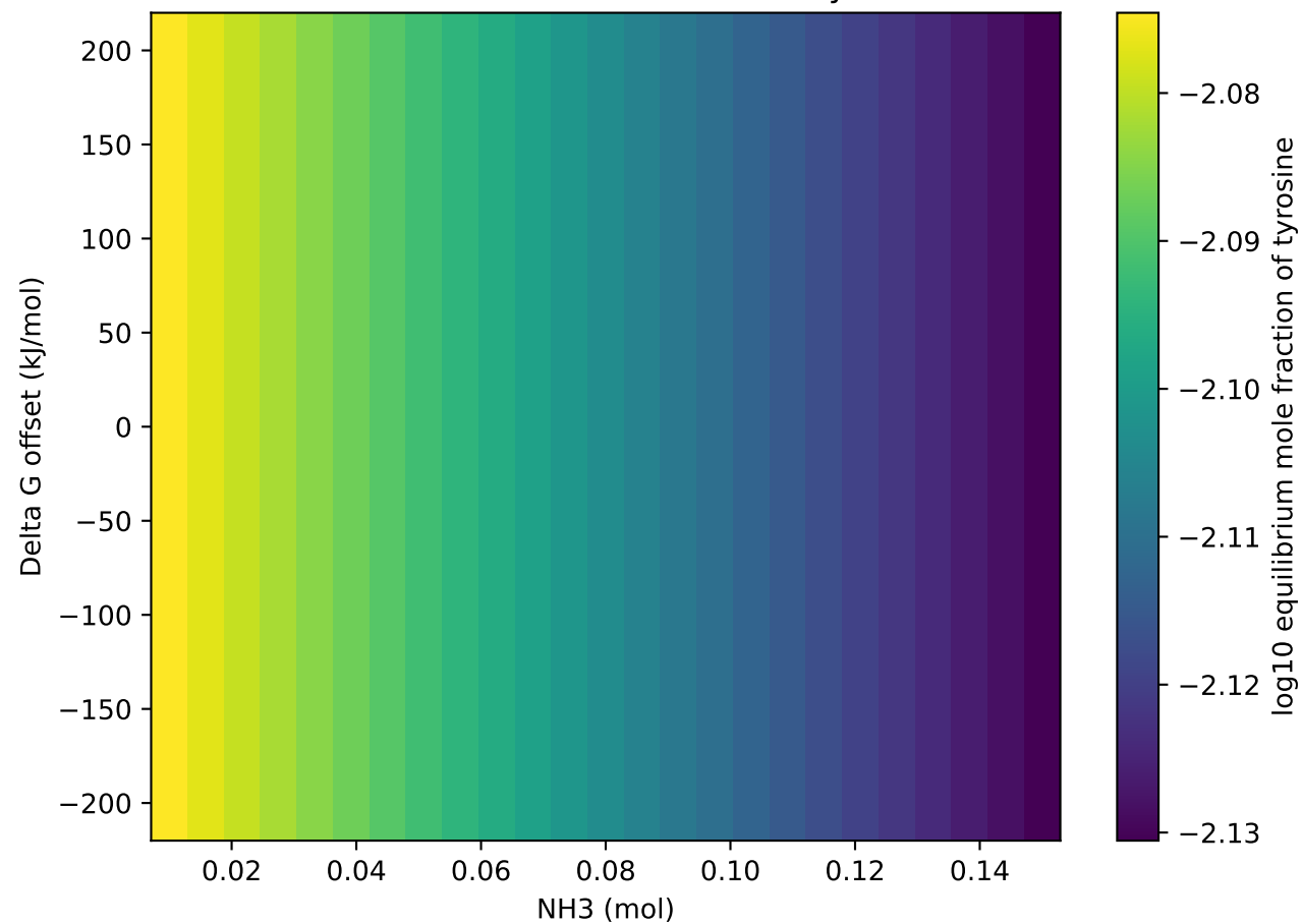
NH 3 threshold vs Gibbs offset for tyrosine
