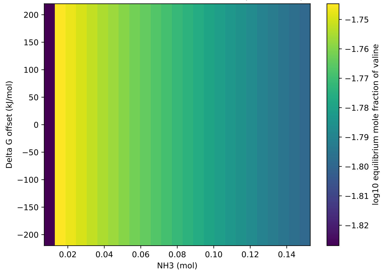
NH 3 threshold vs Gibbs offset for valine (autoscaled)
