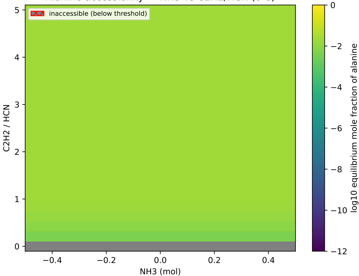
Alanine accessibility — NH 3 vs C 2 H 2 /HCN (0 C)
