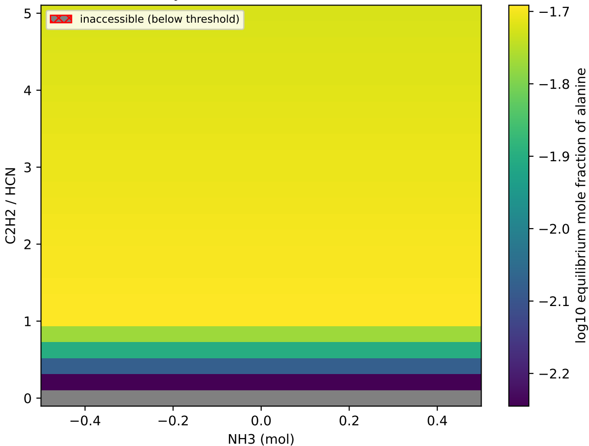
Alanine accessibility — NH 3 vs C 2 H 2 /HCN (0 C) (autoscaled)
