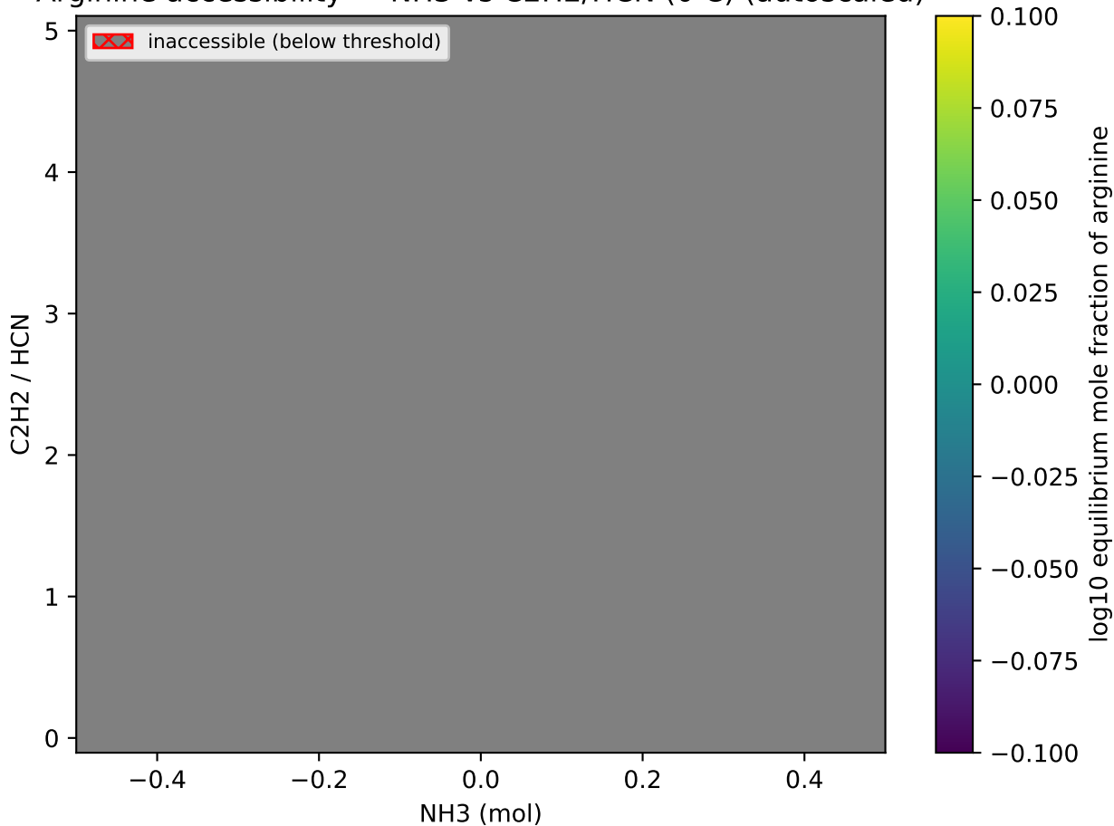
Arginine accessibility — NH3 vs C2H2/HCN (0 C) (autoscaled)
