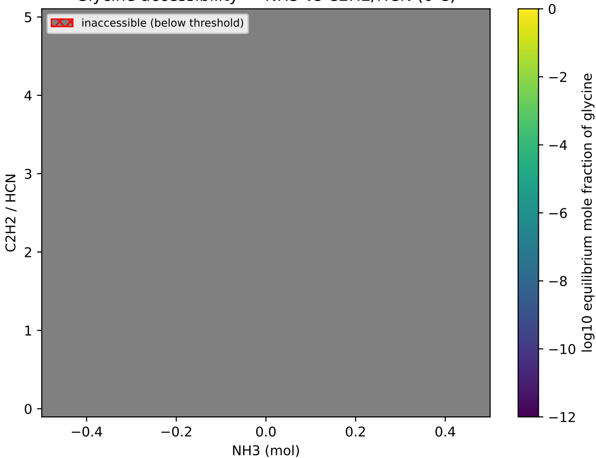
Glycine accessibility — NH 3 vs C 2 H 2 /HCN (0 C)
