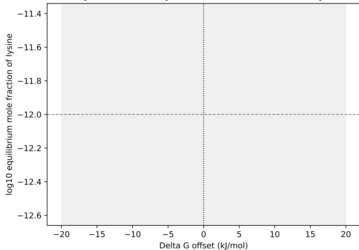
Lysine accessibility vs Gibbs offset (fixed inventory)
