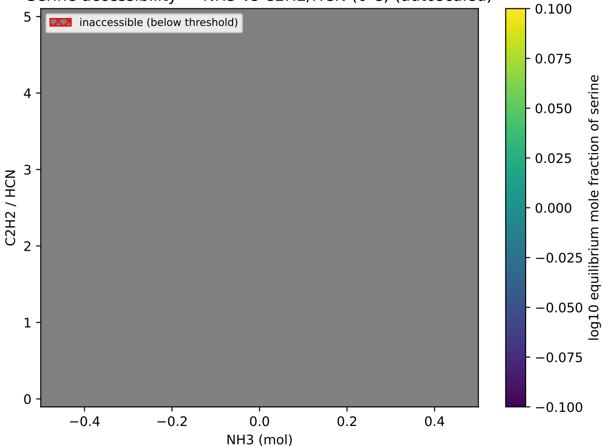
Serine accessibility — NH3 vs C2H2/HCN (0 C) (autoscaled)
