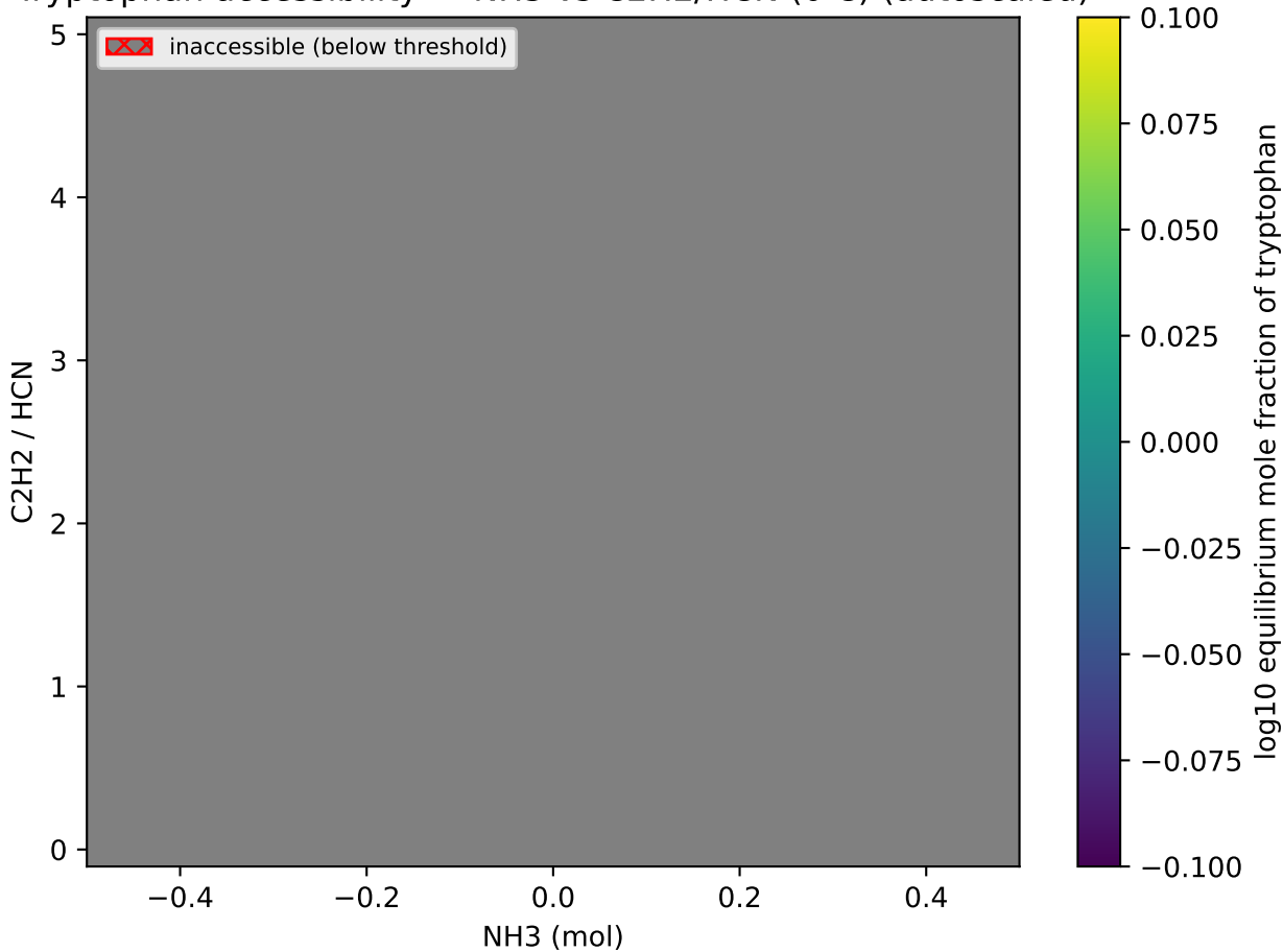
Tryptophan accessibility — NH 3 vs C 2 H 2 /HCN (0 C) (autoscaled)
