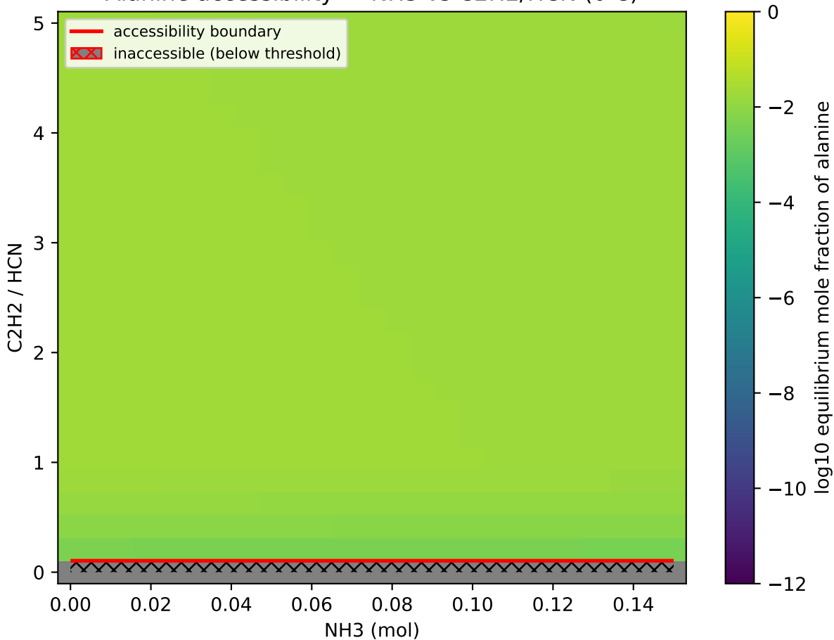
Alanine accessibility — NH3 vs C2H2/HCN (0 C)
