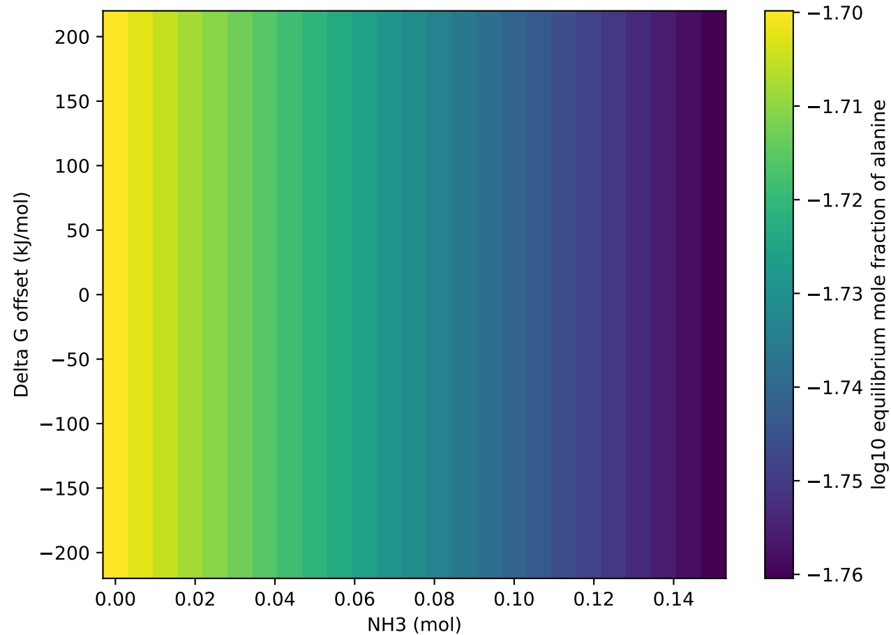
NH 3 threshold vs Gibbs offset for alanine
