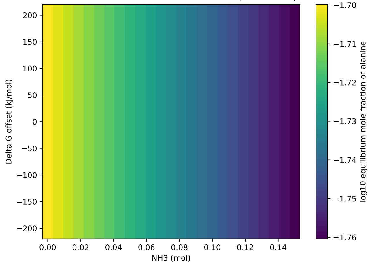
NH 3 threshold vs Gibbs offset for alanine (autoscaled)
