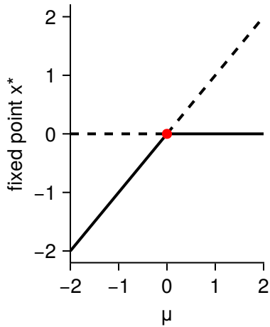
(b) transcritical
