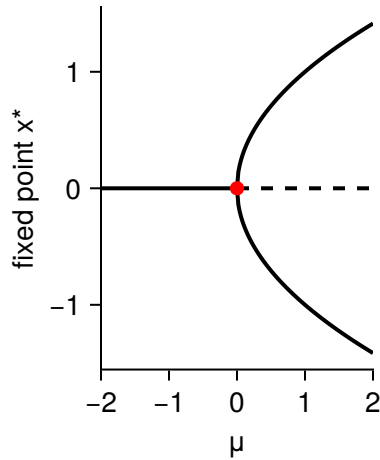
(c) supercritical pitchfork
