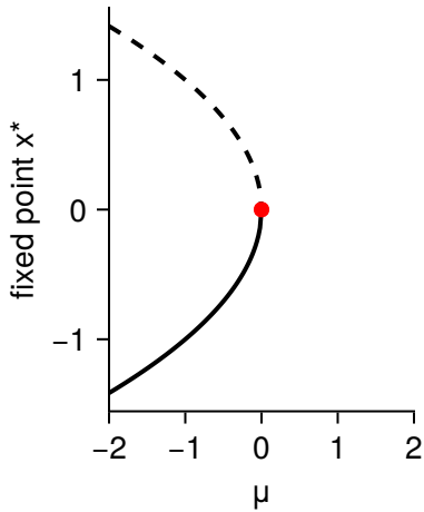
(a) saddle-node
