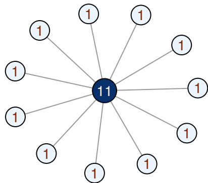
(a) star (N=12)
