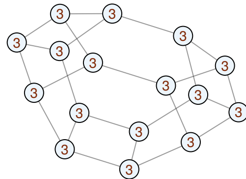
(c) random regular (N=16)
