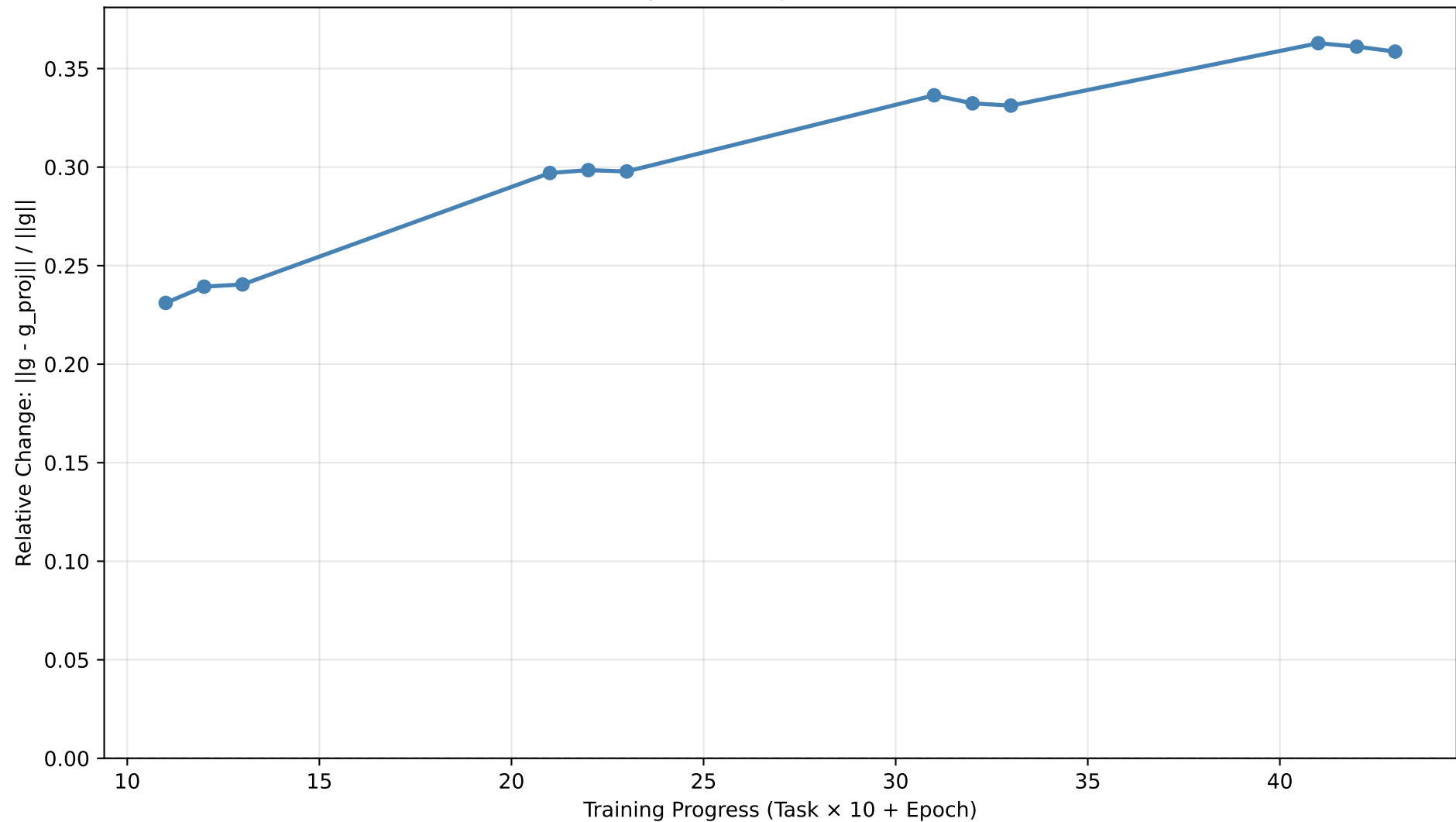
OGD: Impact of Projection on Gradient
