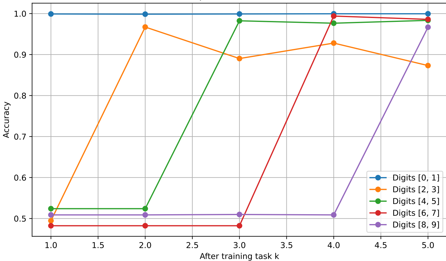
Split MNIST — OGD
