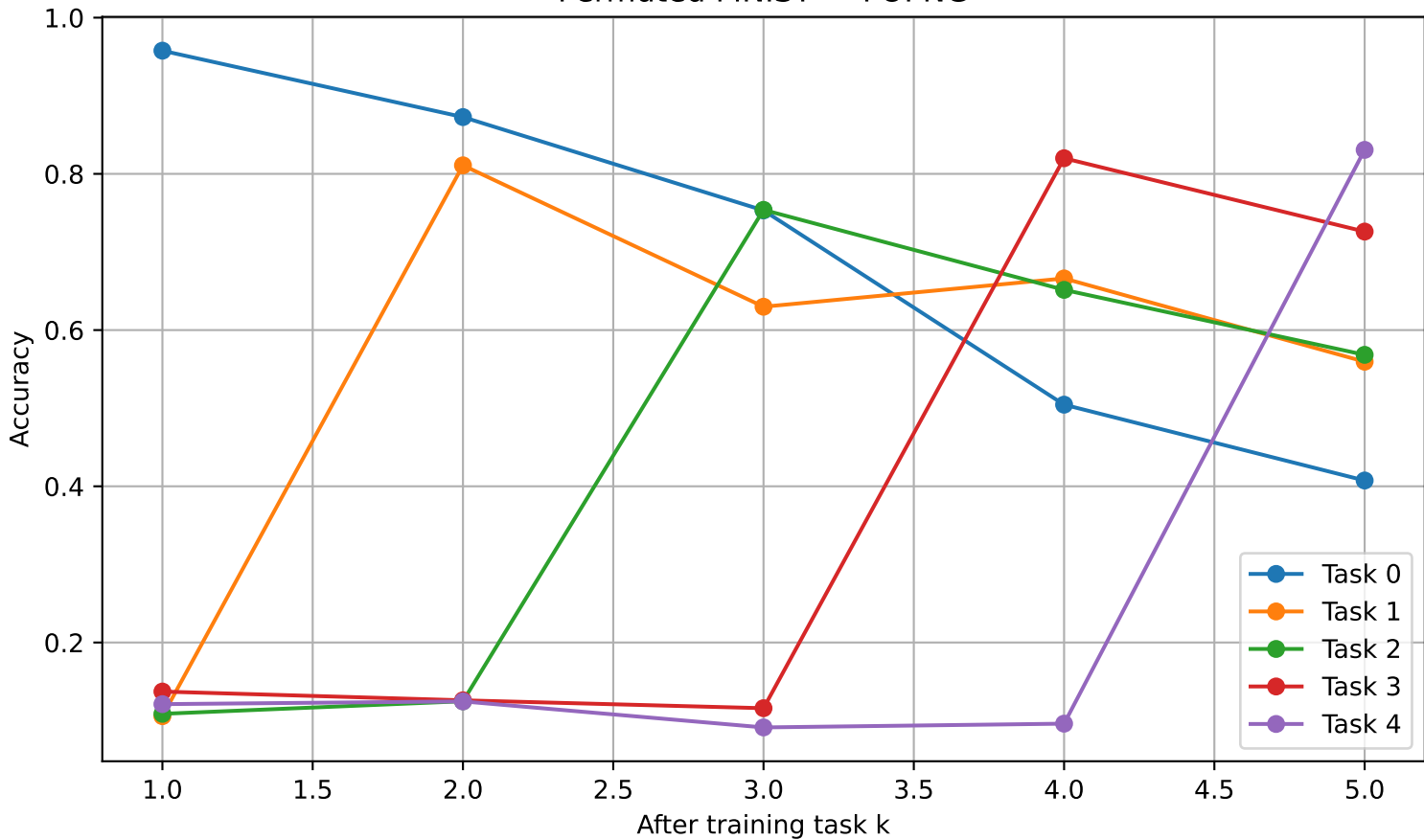
Permuted MNIST — FOPNG
