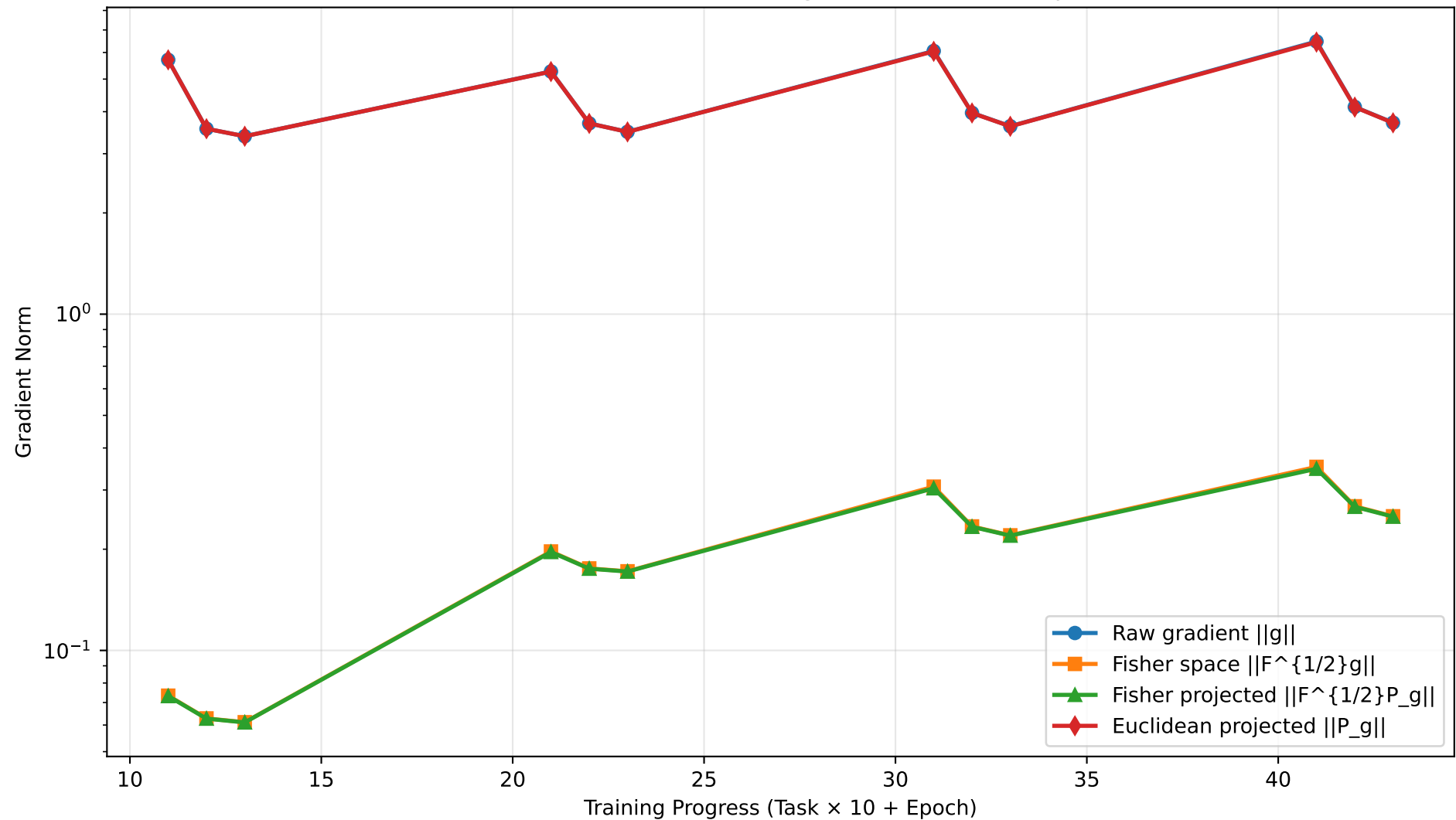
FOPNG Gradient Norms Through Transformation Pipeline
