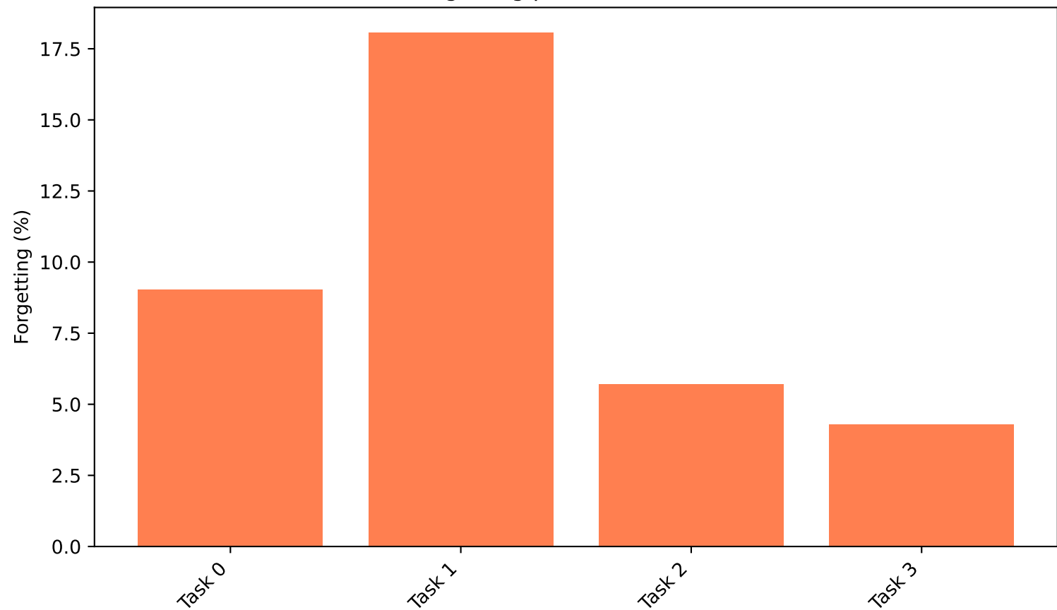
Forgetting per Task — FOPNG
