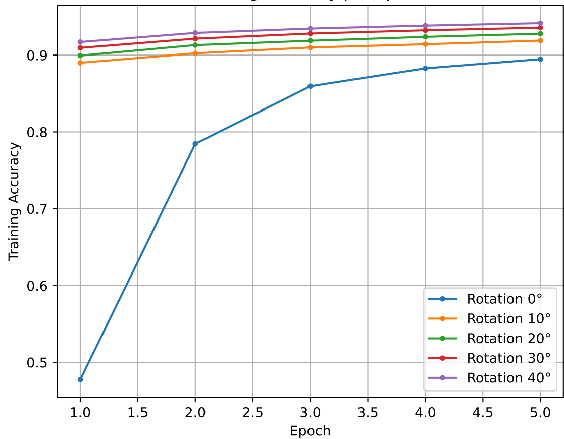
Training Accuracy per Epoch
