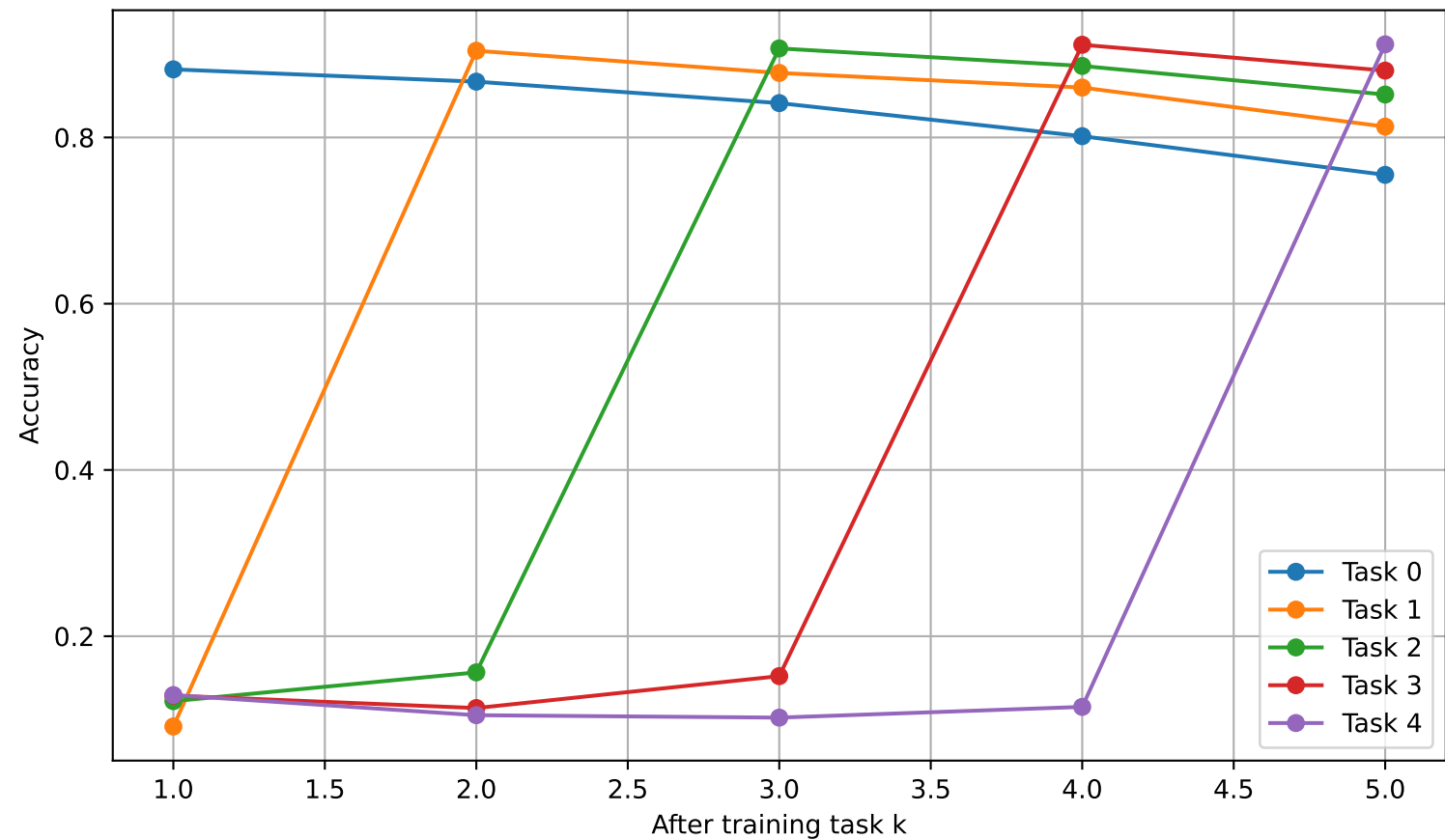
Permuted MNIST — OGD
