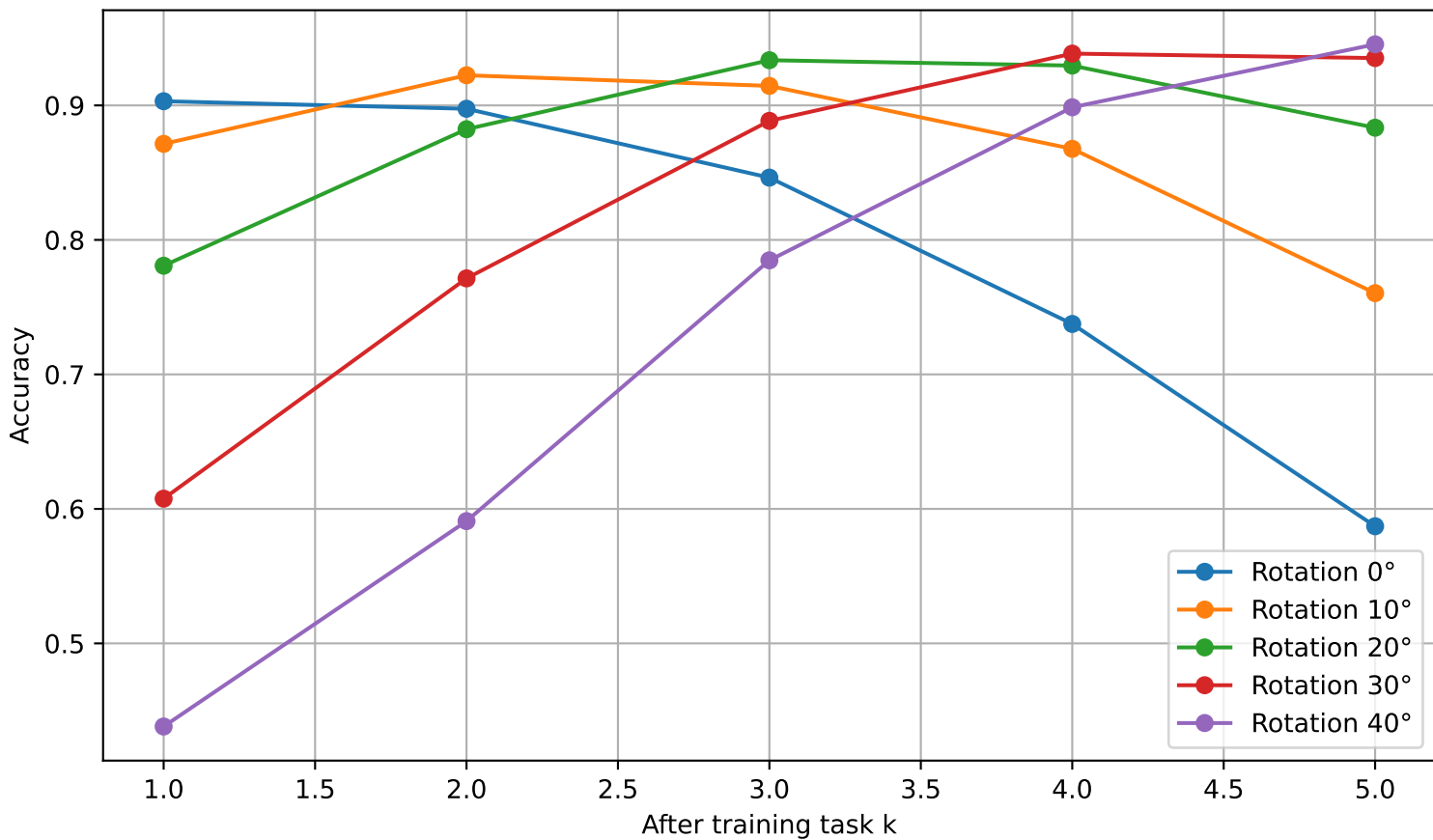
Rotated MNIST — SGD
