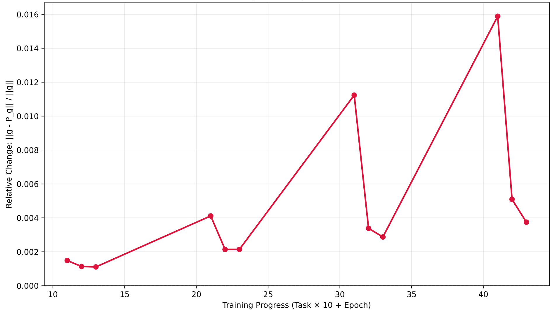
FOPNG: Impact of Projection on Gradient
