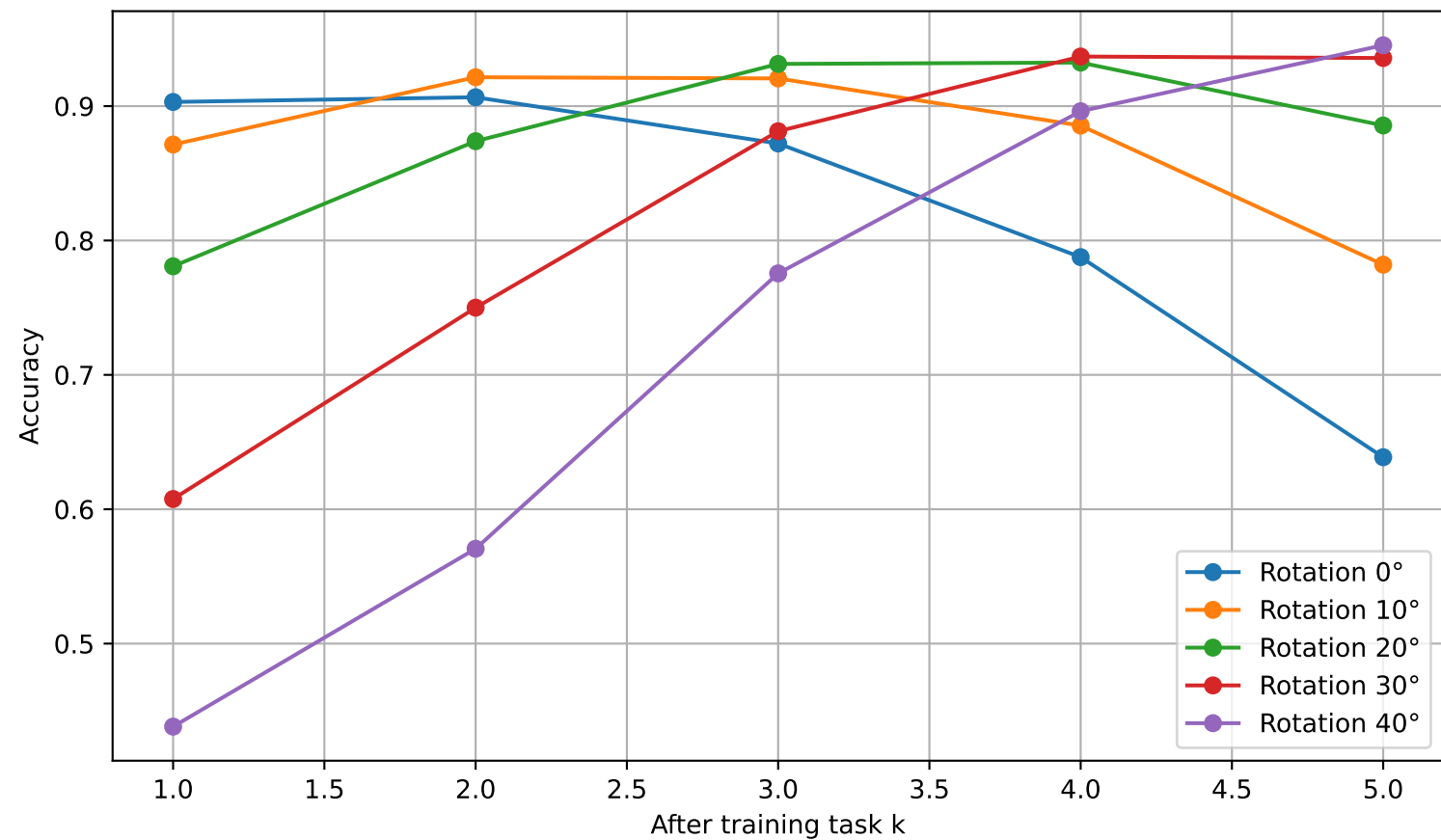
Rotated MNIST — OGD
