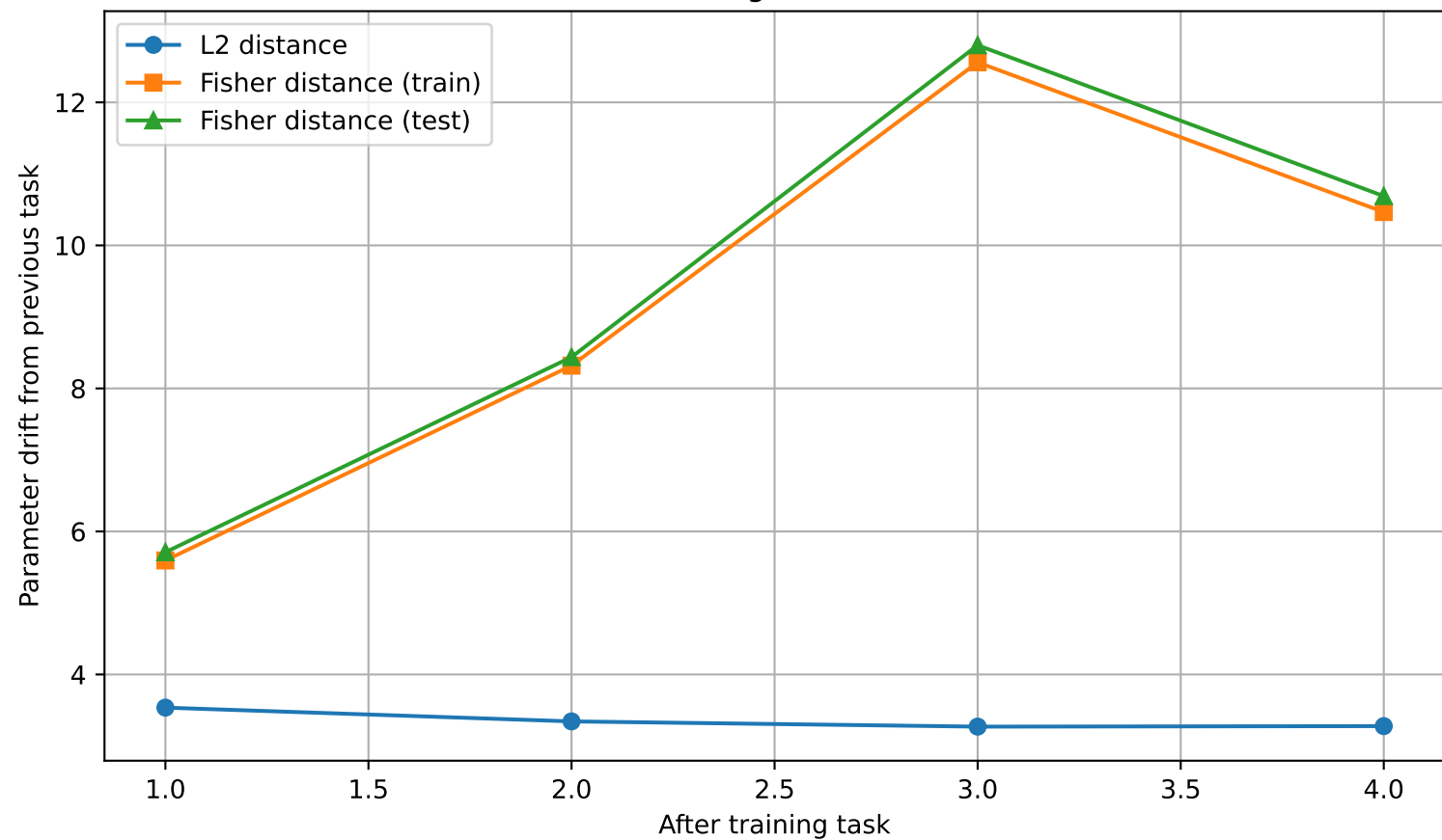
Distribution Change Over Time — SGD
