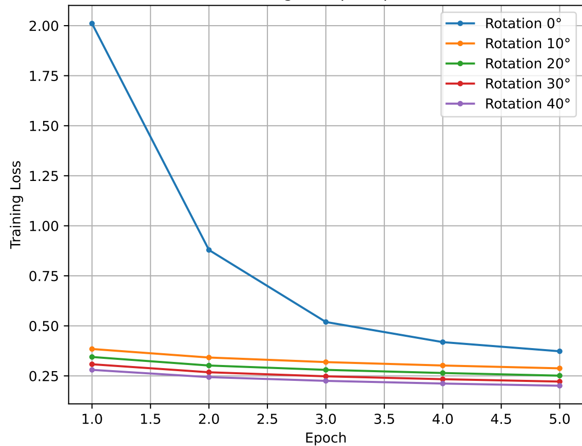
Training Loss per Epoch
