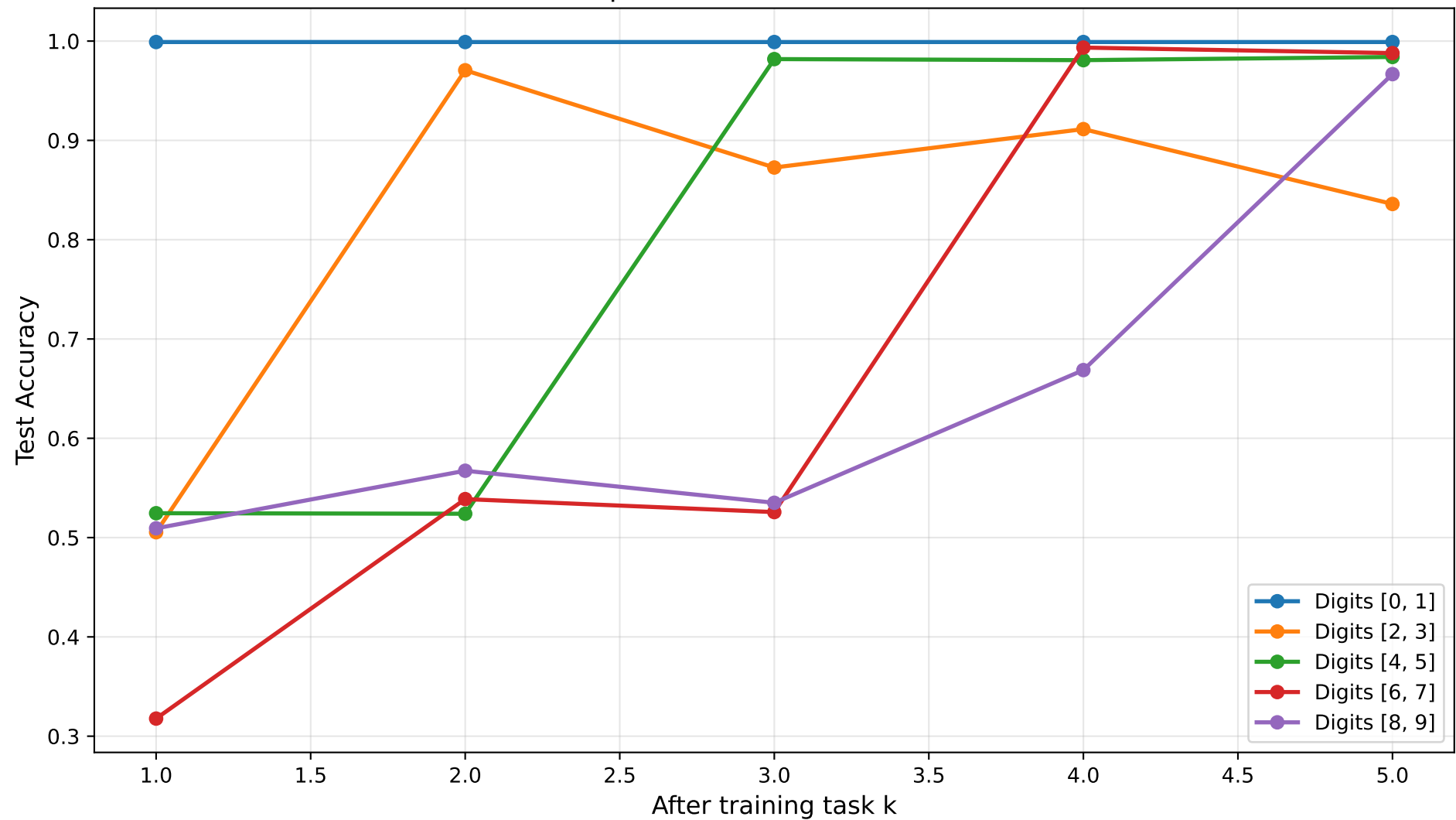
Split MNIST — OGD (Test)
