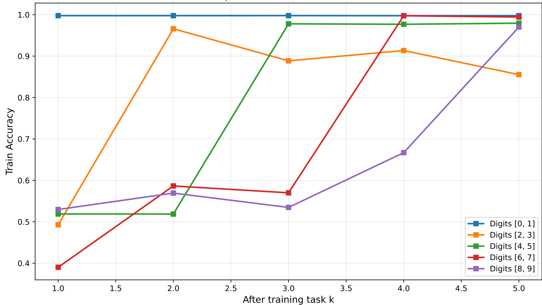
Split MNIST — OGD (Train)
