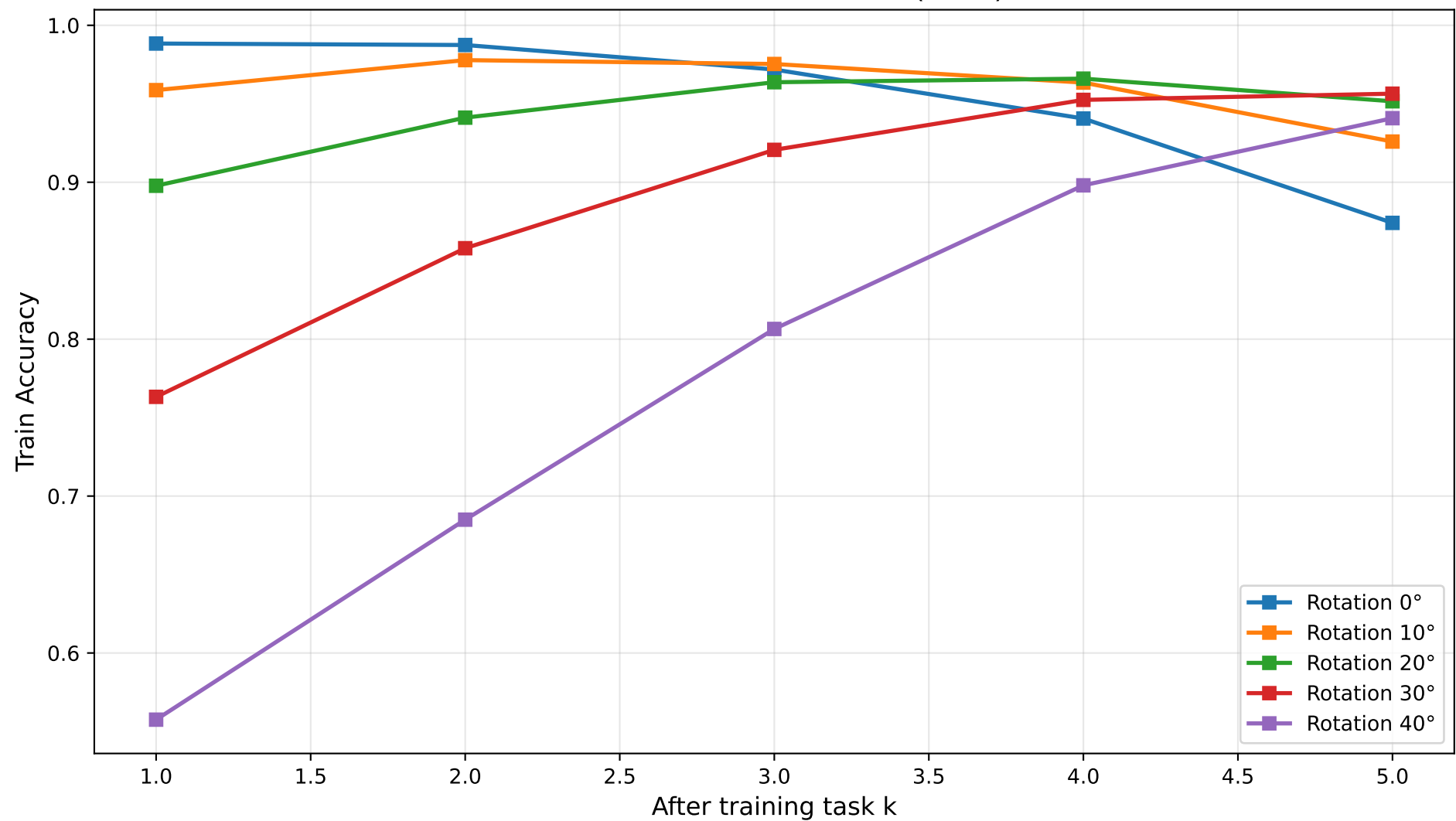
Rotated MNIST — FOPNG (Train)
