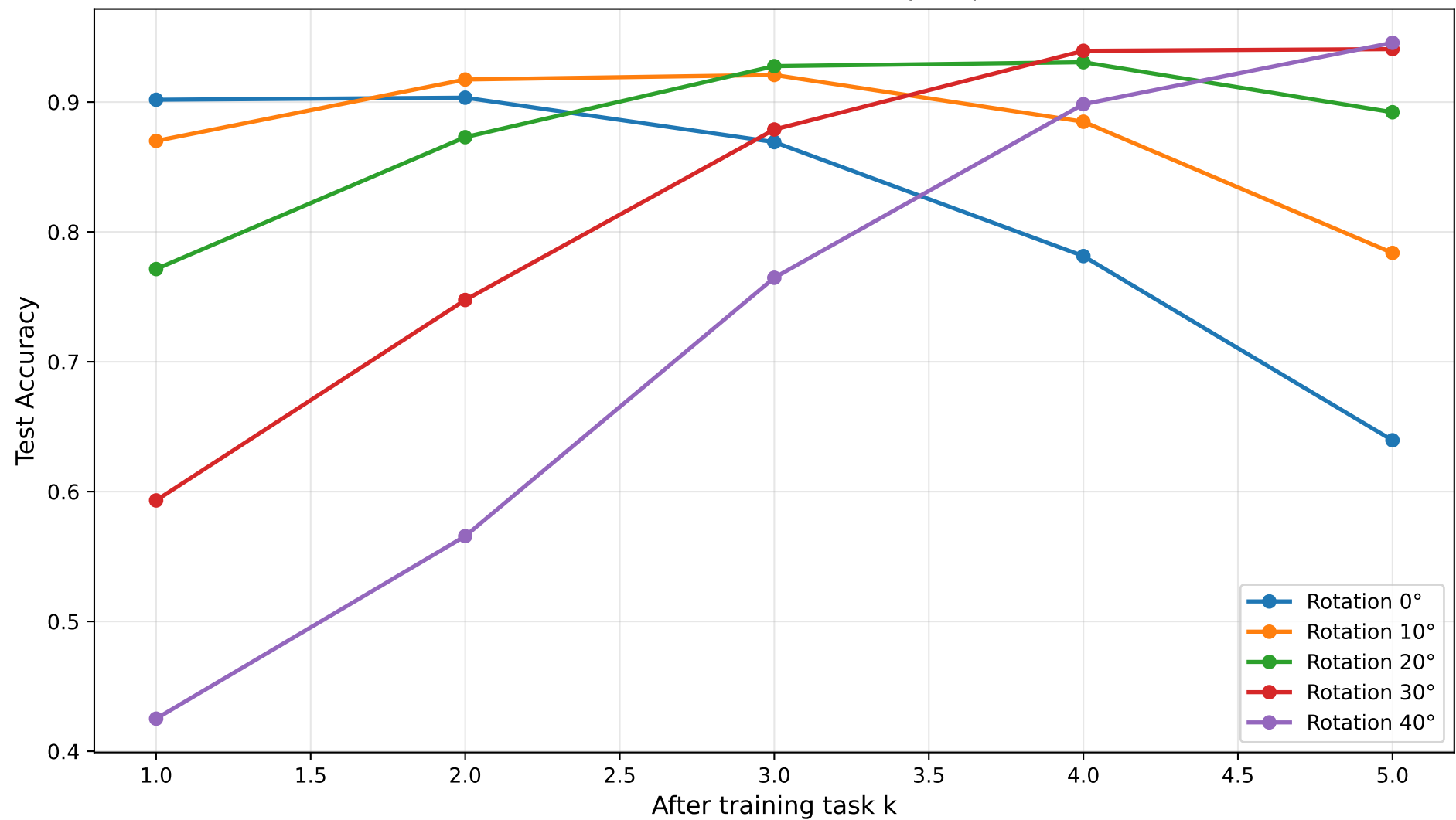
Rotated MNIST — OGD (Test)
