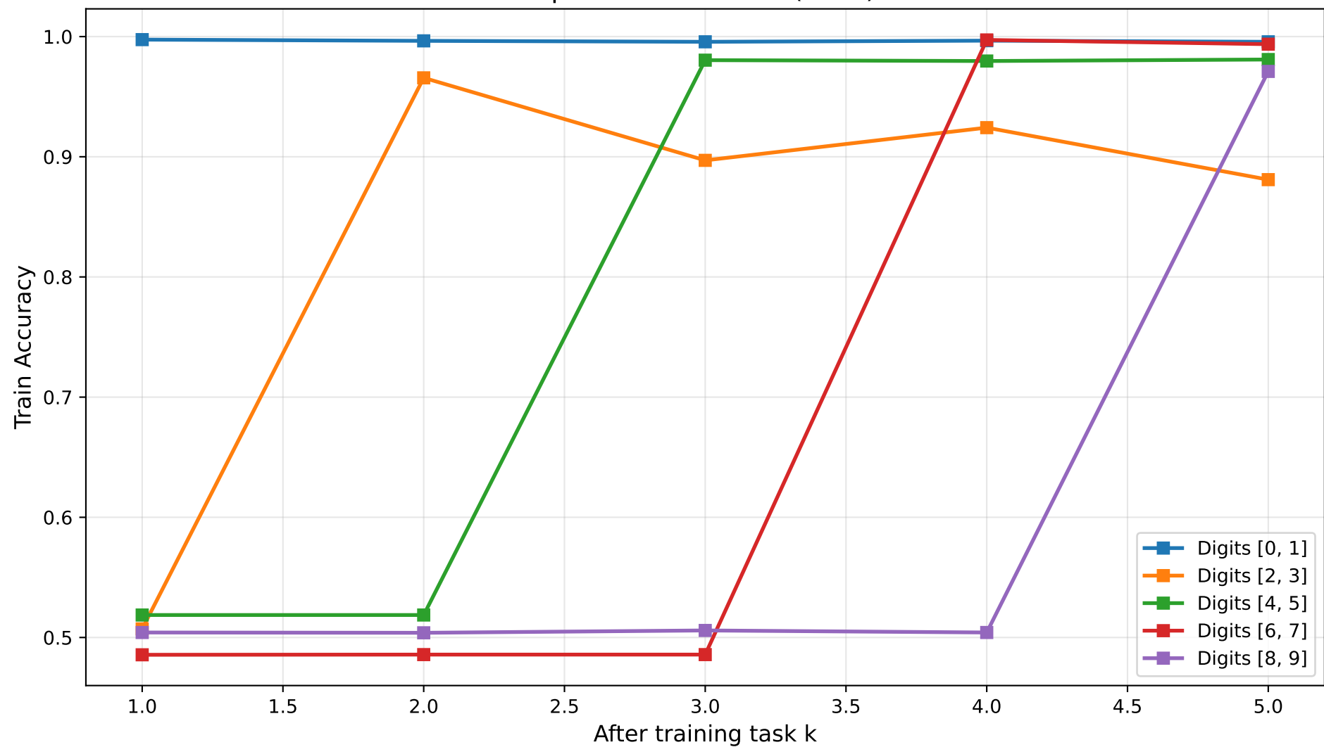
Split MNIST — SGD (Train)
