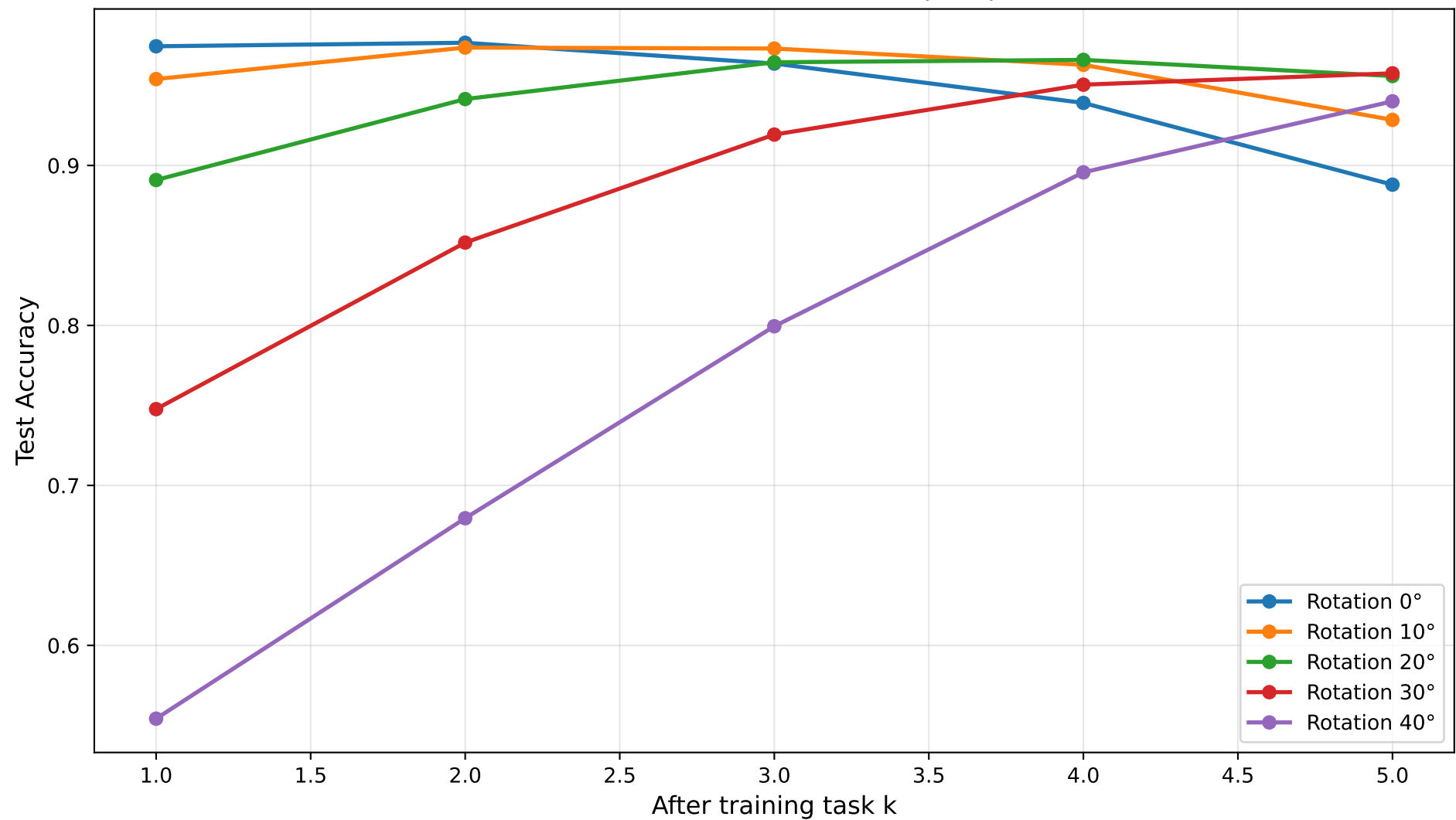
Rotated MNIST — FOPNG (Test)
