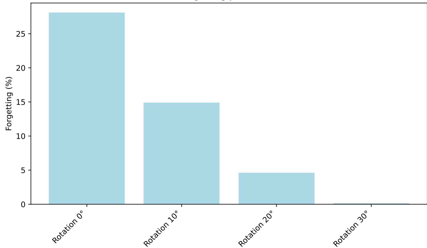
Train Forgetting per Task — OGD
