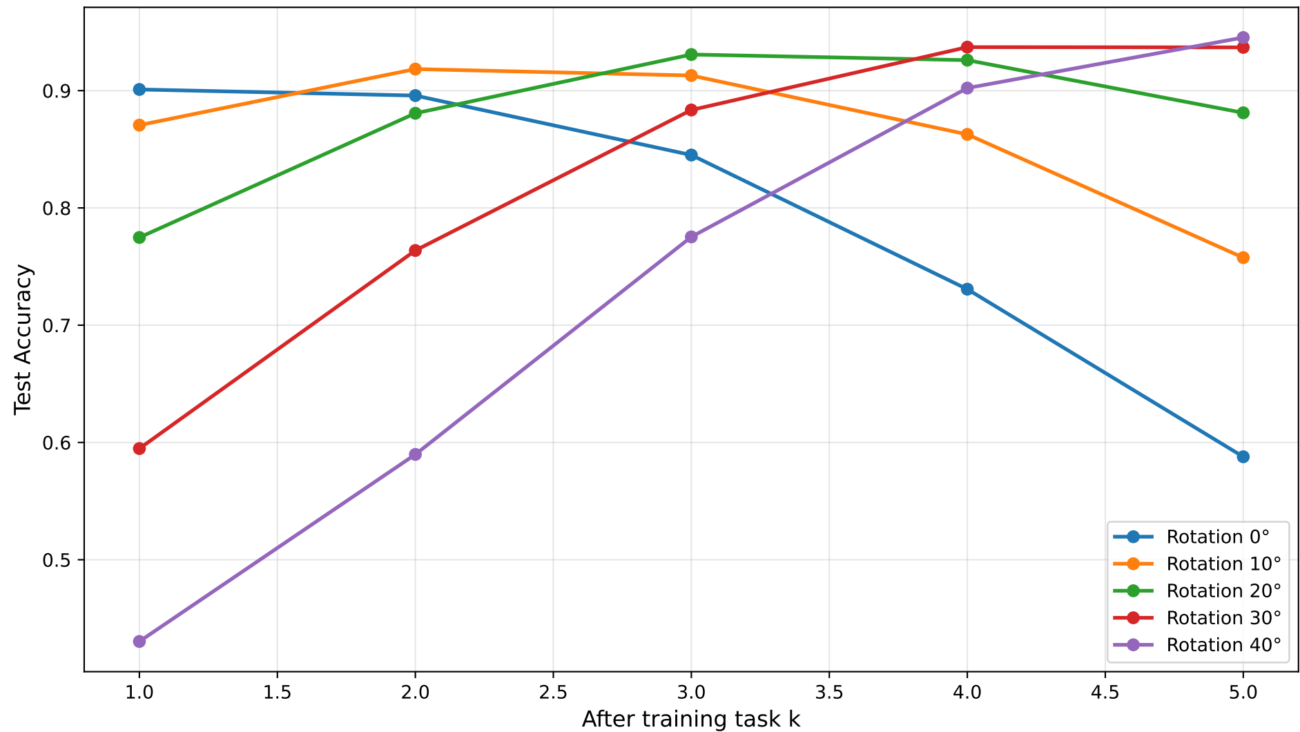
Rotated MNIST — SGD (Test)
