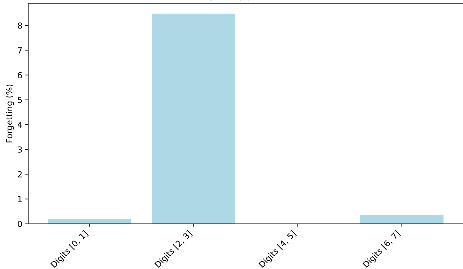
Train Forgetting per Task — SGD
