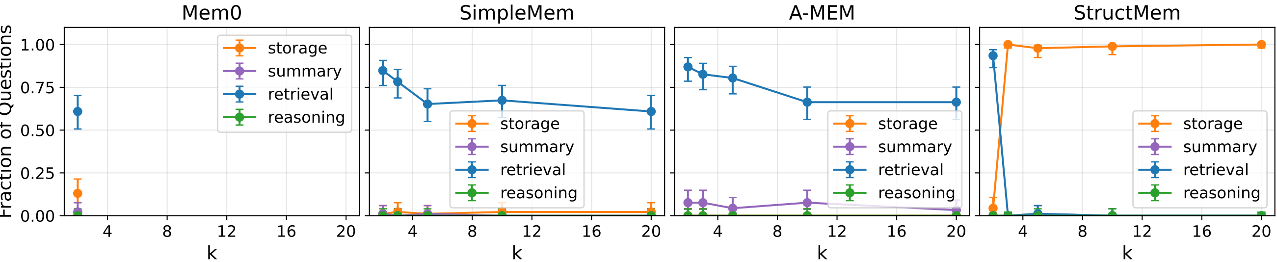
All-error breakdown vs. k — Long-Hop / gemini-3.1
