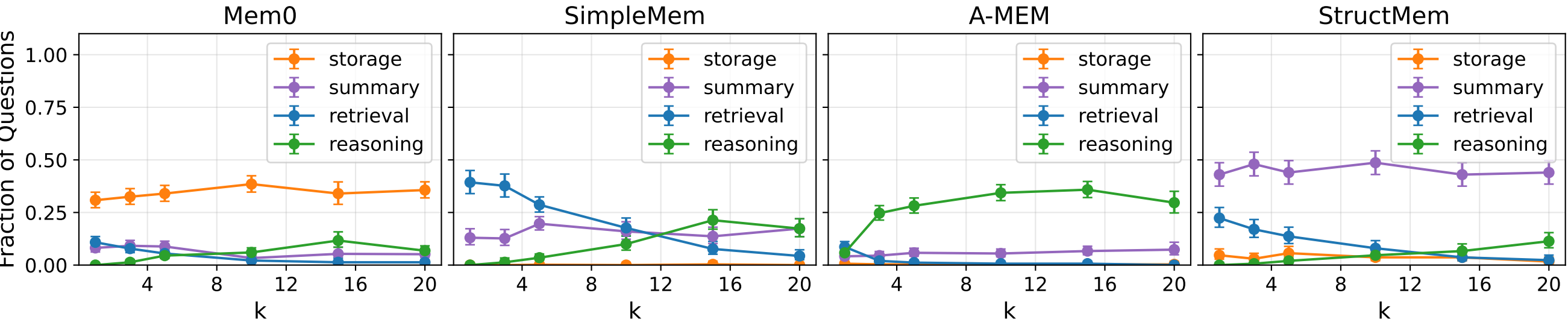
All-error breakdown vs. k — Persona-Retrieval / gpt-4.1-mini
