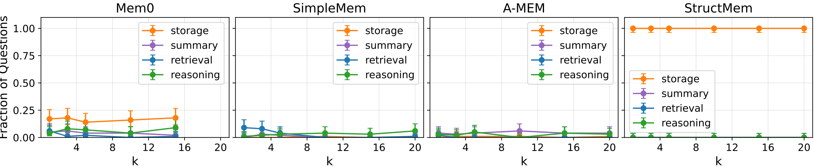
All-error breakdown vs. k — Conditional-Facts / gpt-5.4-mini
