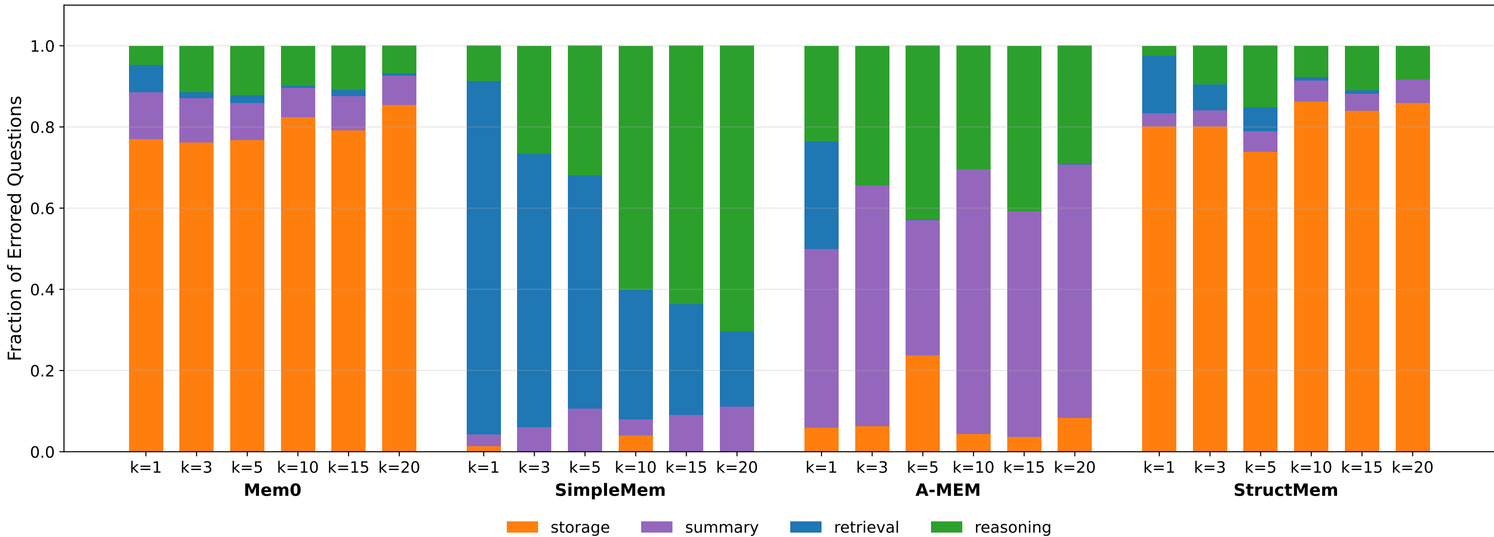
Error breakdown vs. k — Conditional-Facts
