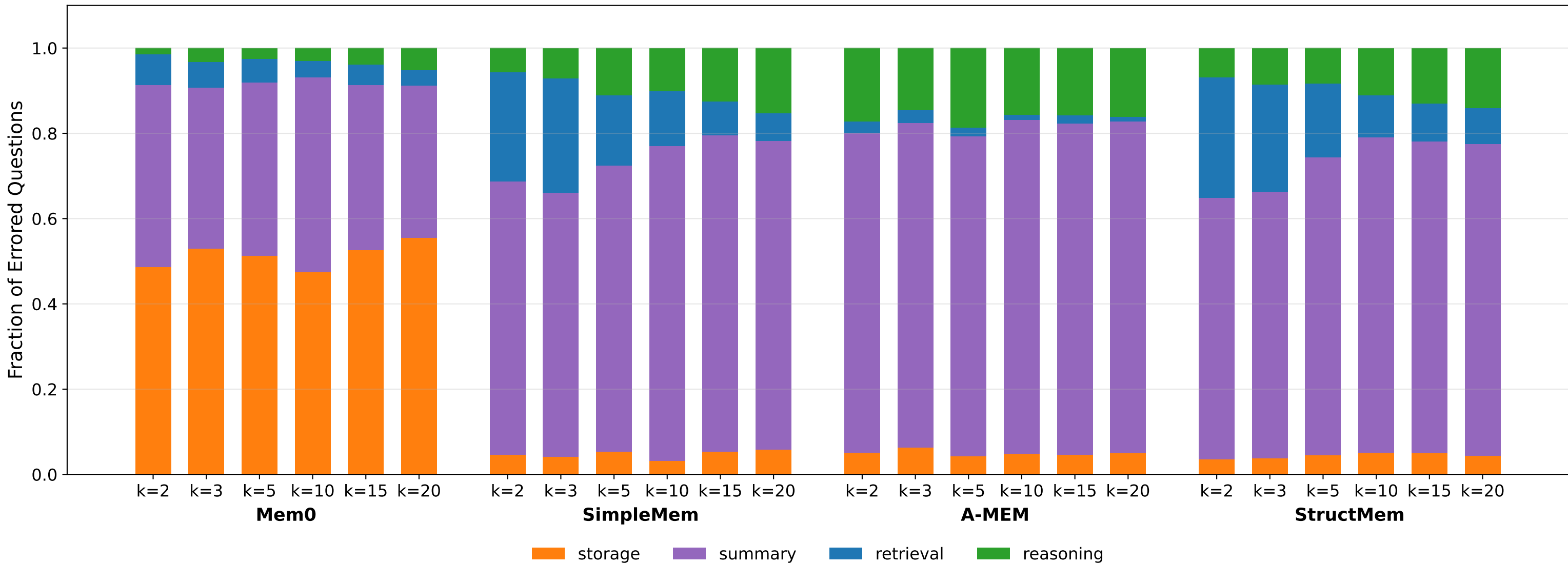
Error breakdown vs. k — Conditional-Facts (Hard)
