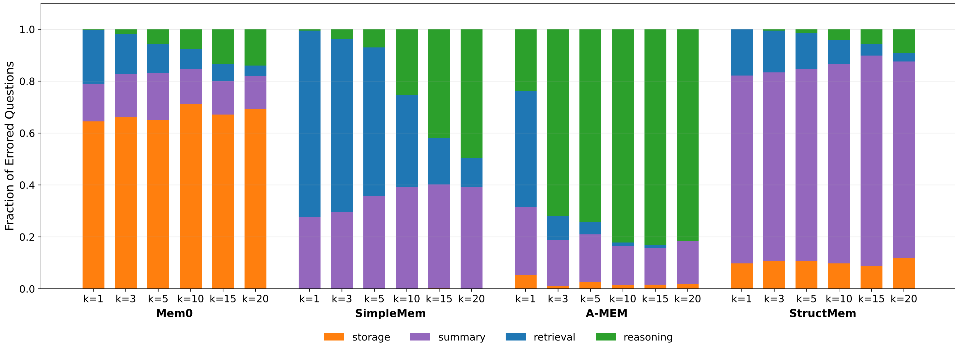
Error breakdown vs. k — Persona-Retrieval
