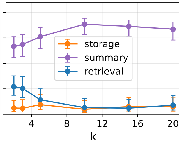
StructMem
