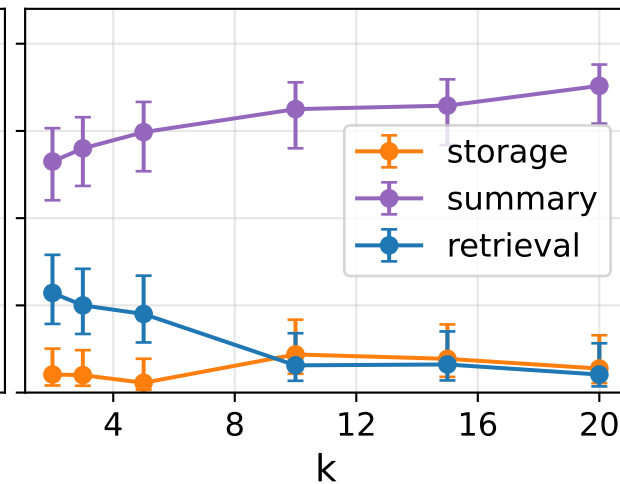
StructMem
