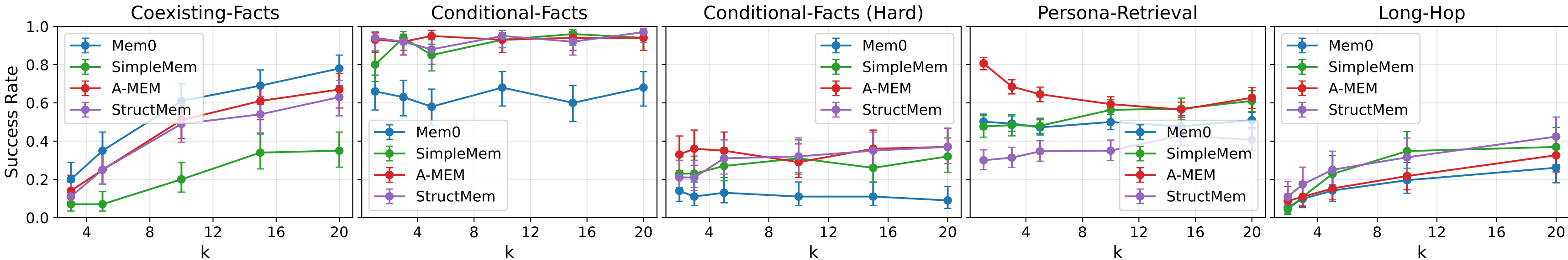
Success rate vs. k — gpt-4.1-mini
