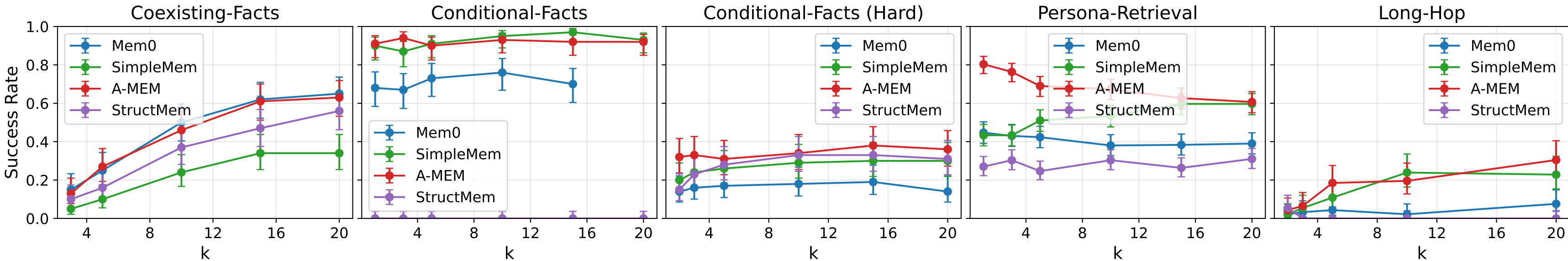
Success rate vs. k — gpt-5.4-mini
