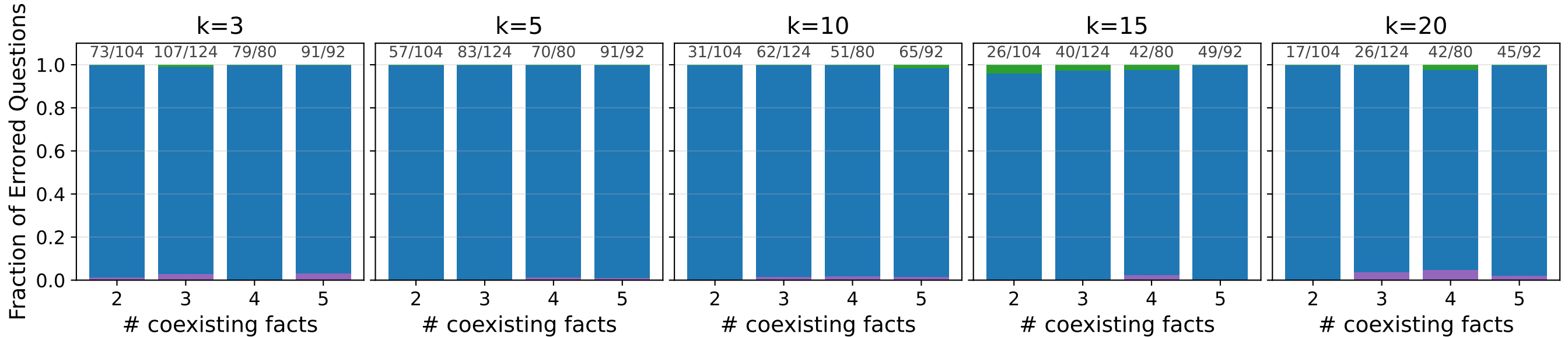
Coexisting-Facts — error breakdown by # facts and k (A-MEM)
