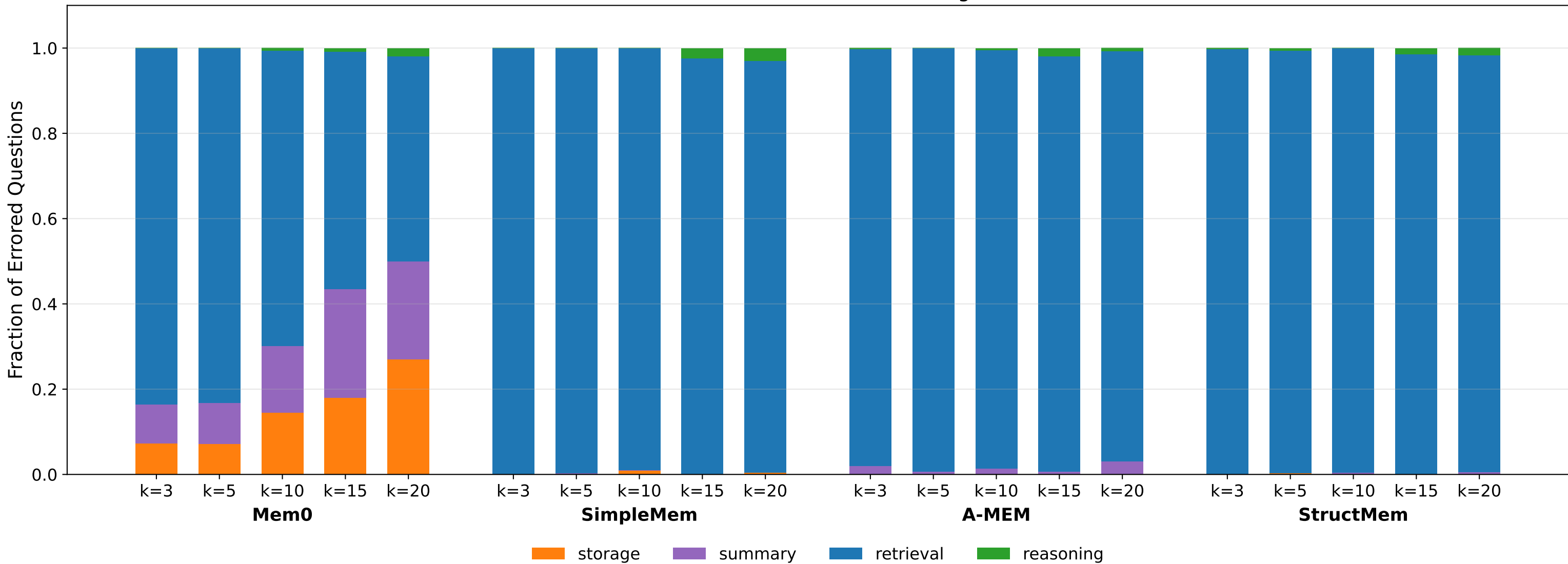
Error breakdown vs. k — Coexisting-Facts
