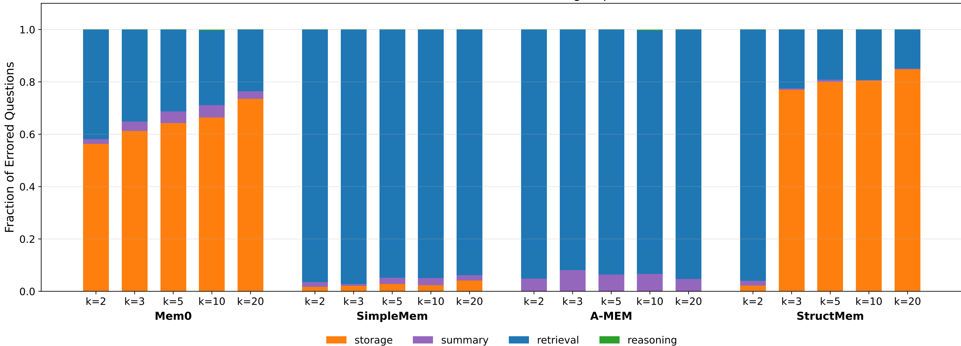
Error breakdown vs. k — Long-Hop
